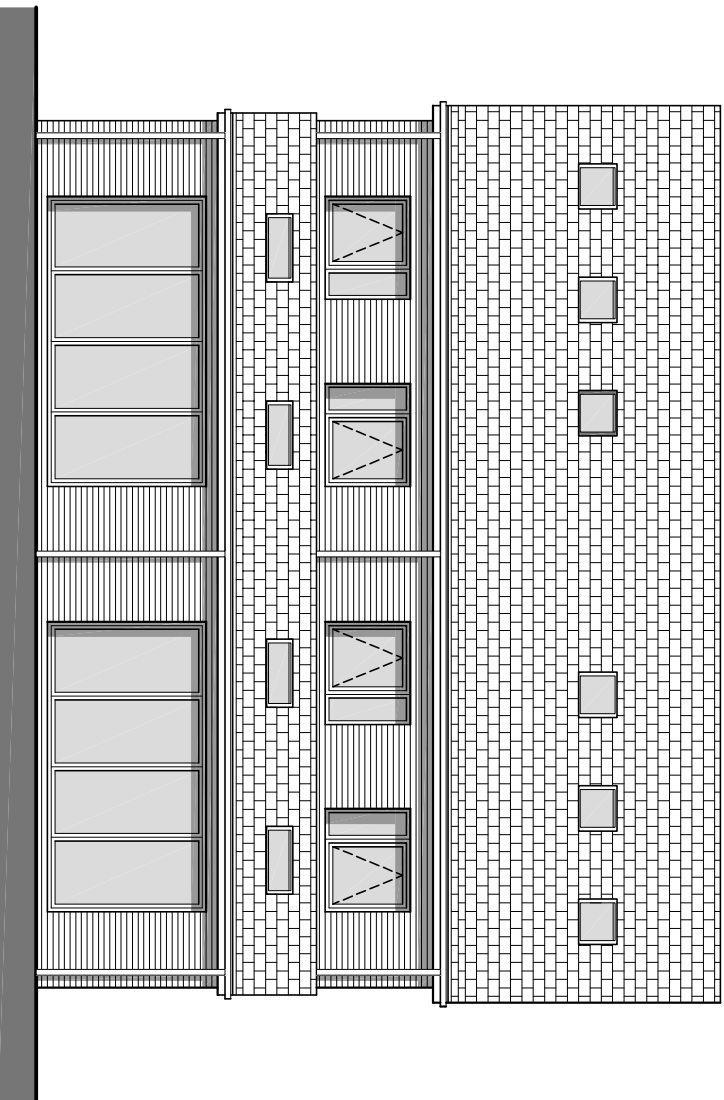
Rear Elevation
