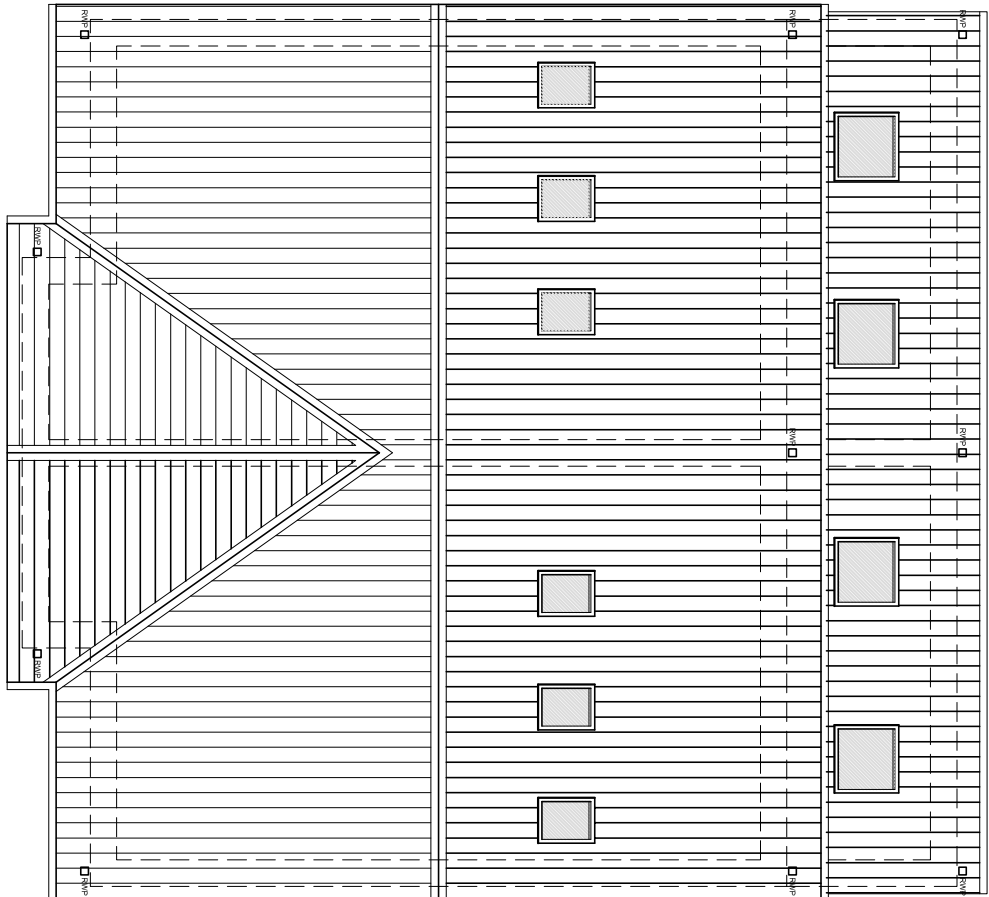
Roof Plan
