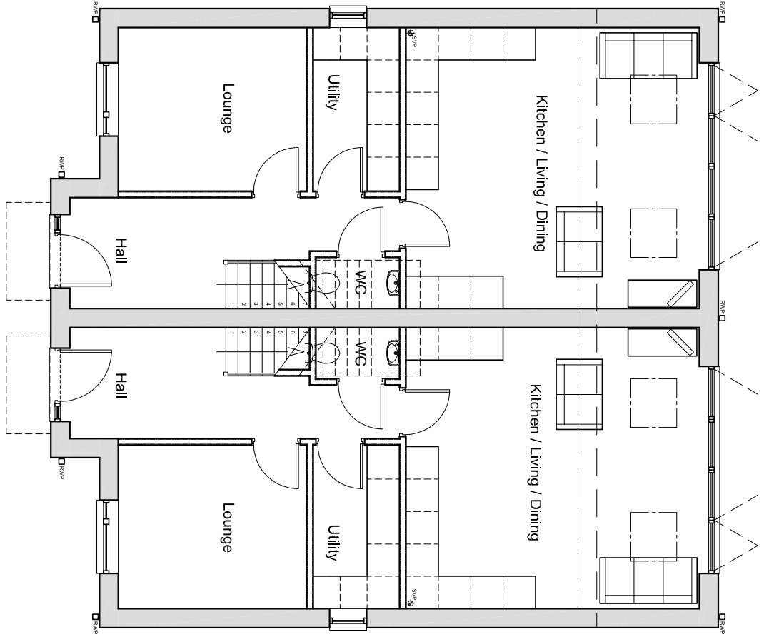
Ground Floor Plan P005 - H27, 28, 31, 32, 35, 36, 39-50 - All Units - 487P - 127sqm
