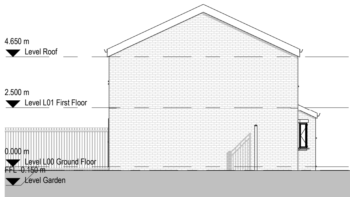
4 Existing North Elevation 1 : 100
