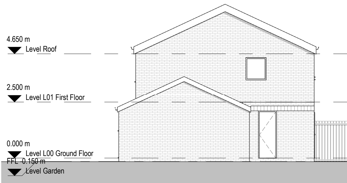
2 Existing South Elevation 1 : 100
