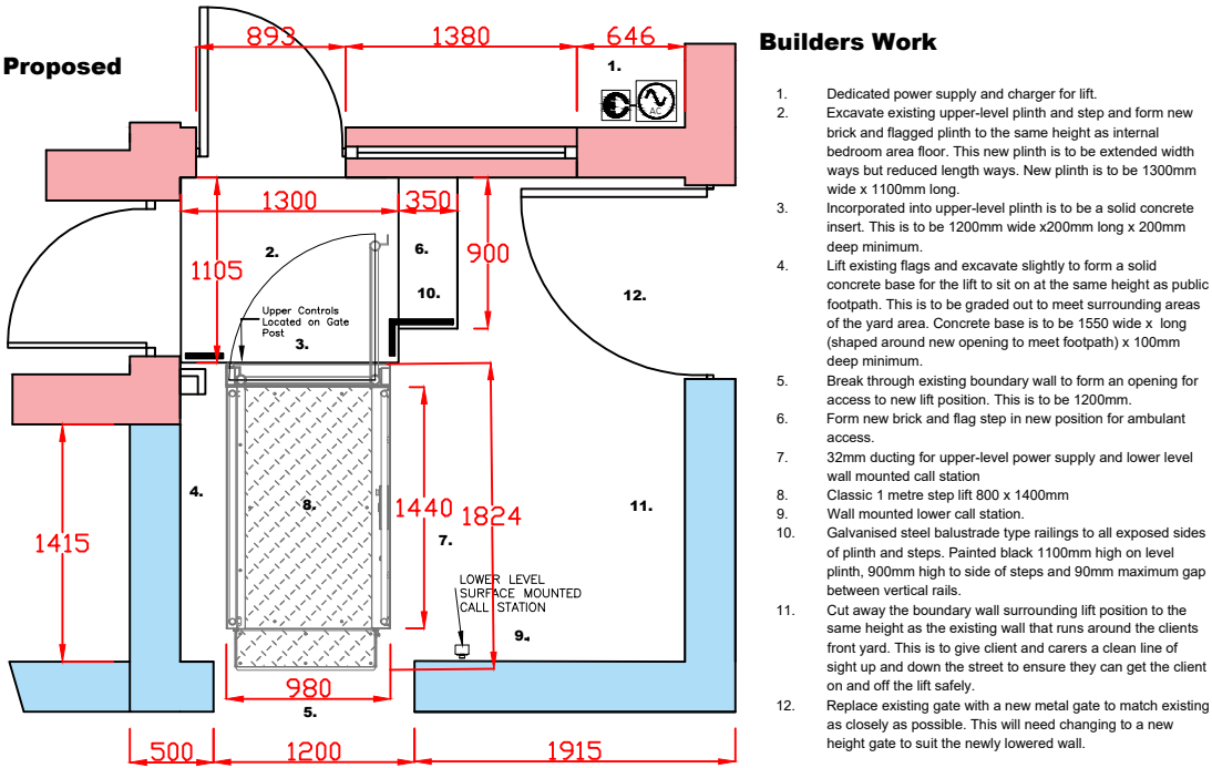
PROPOSED PLAN LAYOUT
