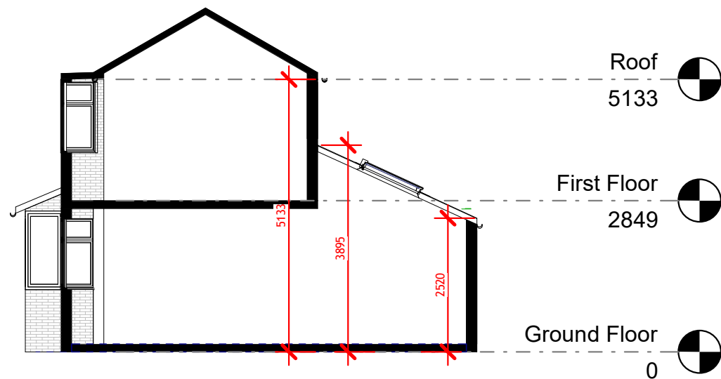
1 Section 1-1 Proposed 1 : 100
