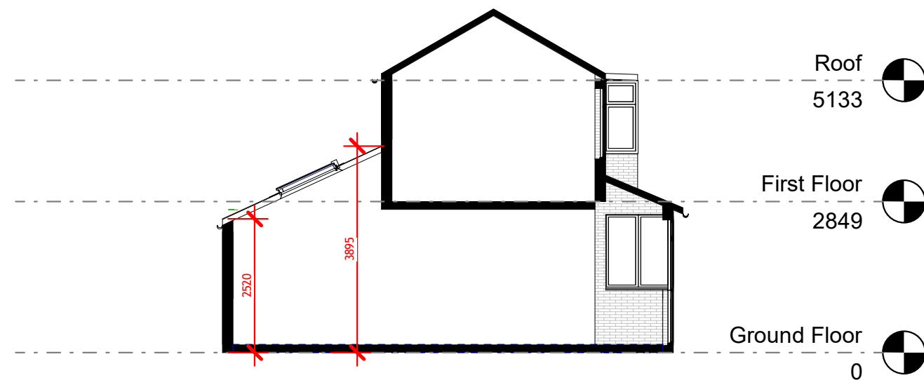
2 Section 2-2 Proposed 1 : 100
