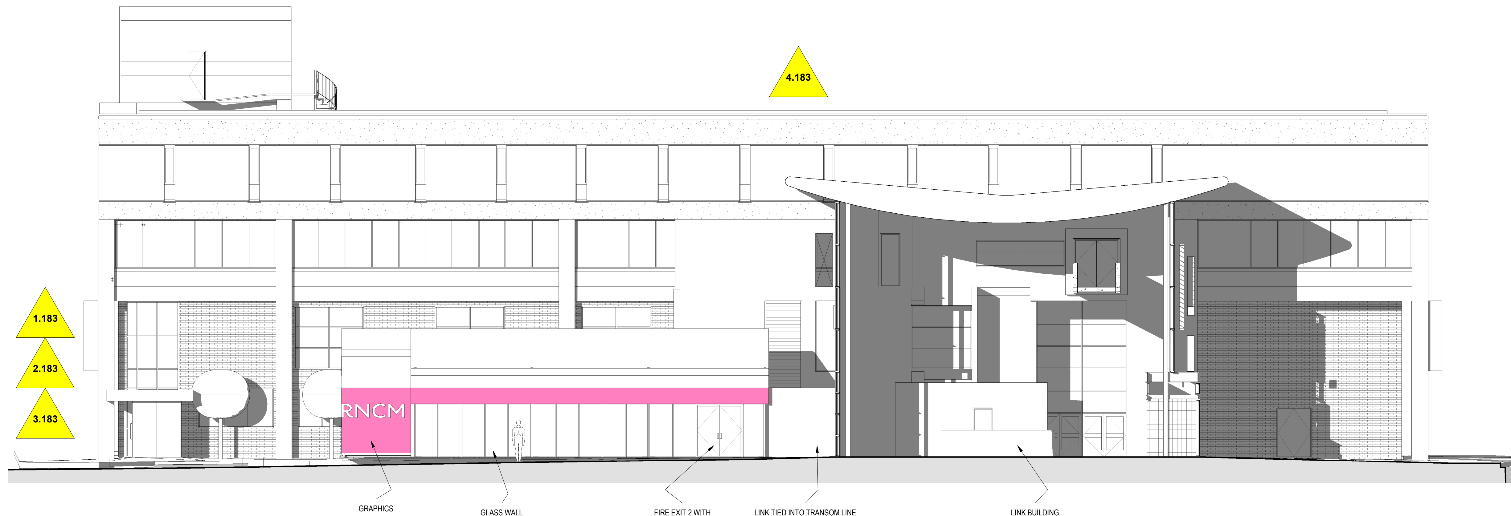
2 Section 2_PHASE 18_3 1 : 100
