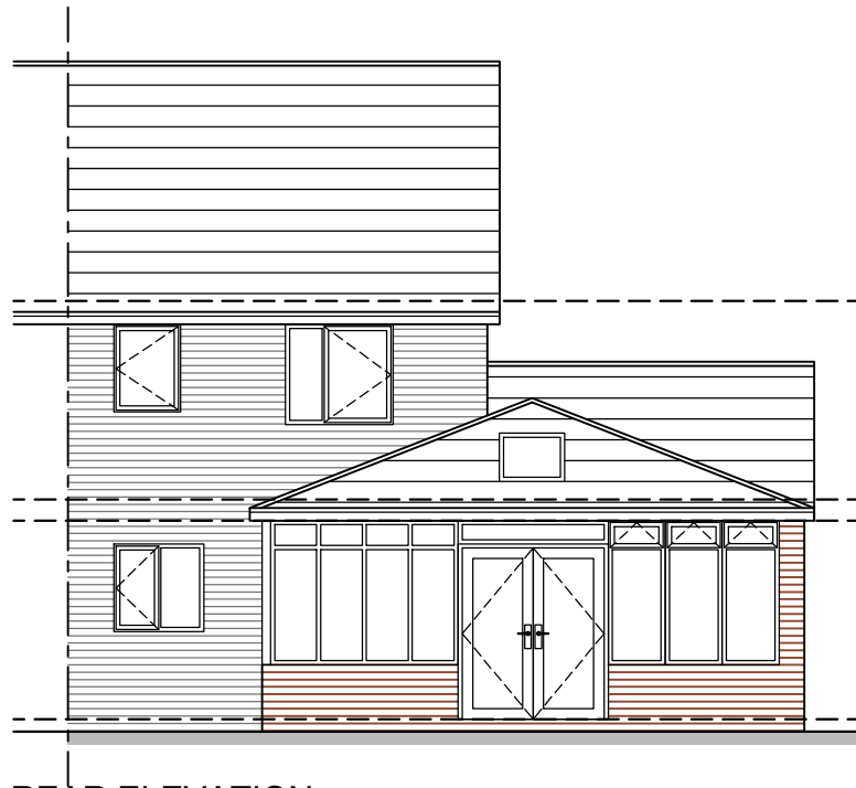
REAR ELEVATION
