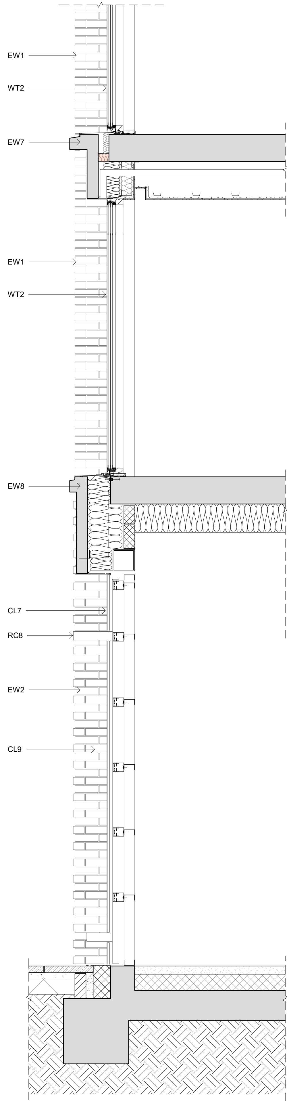
1-20 Detail Sections - Refuse Store_Planning 1 : 20
