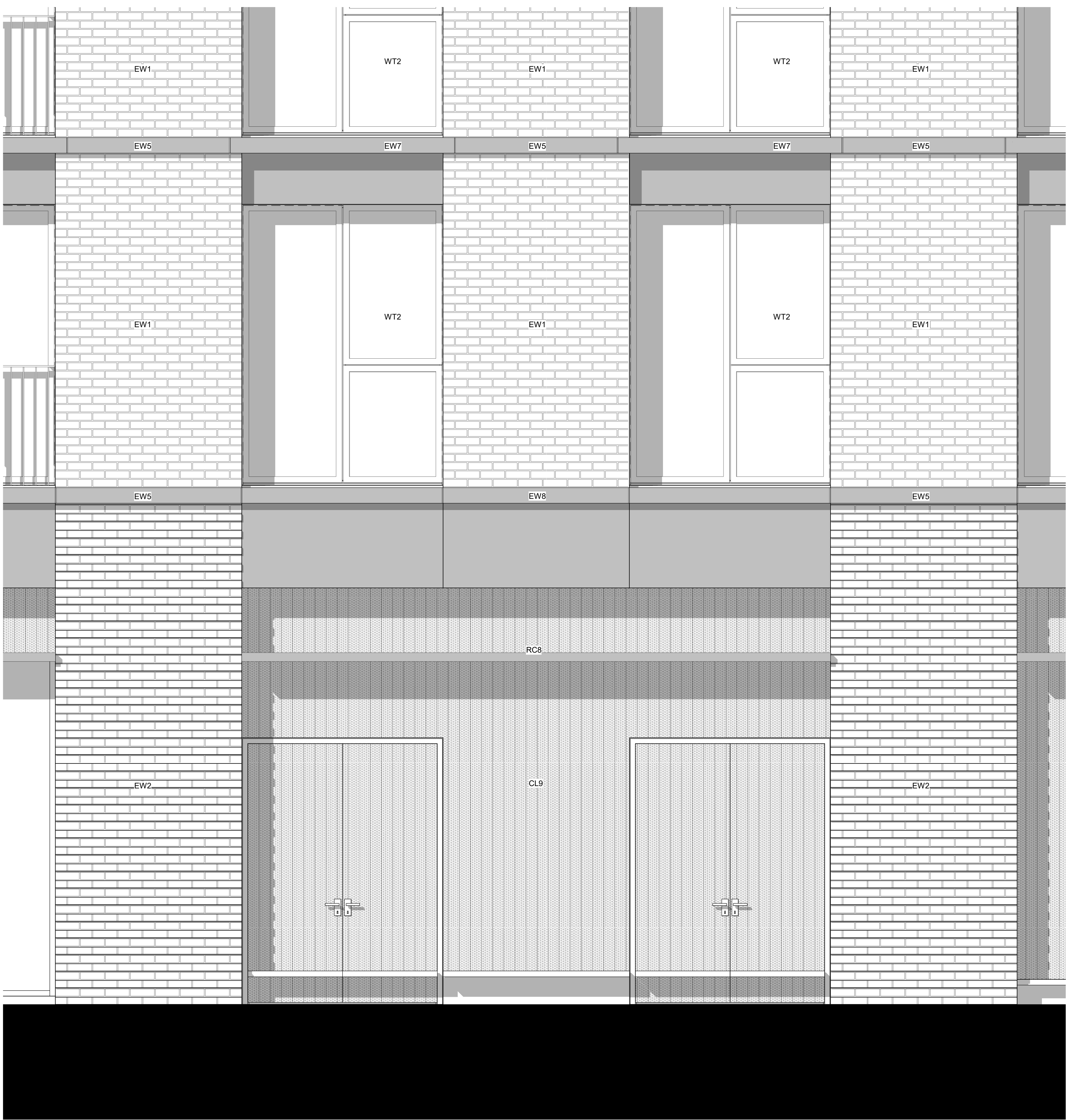
Refuse Store & Typical Residential Window_Planning 1 : 20
