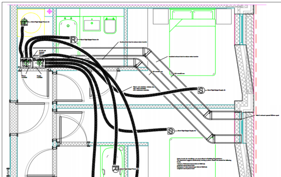
Typical Residential MVHR Layout (c/o Wright Investments)
