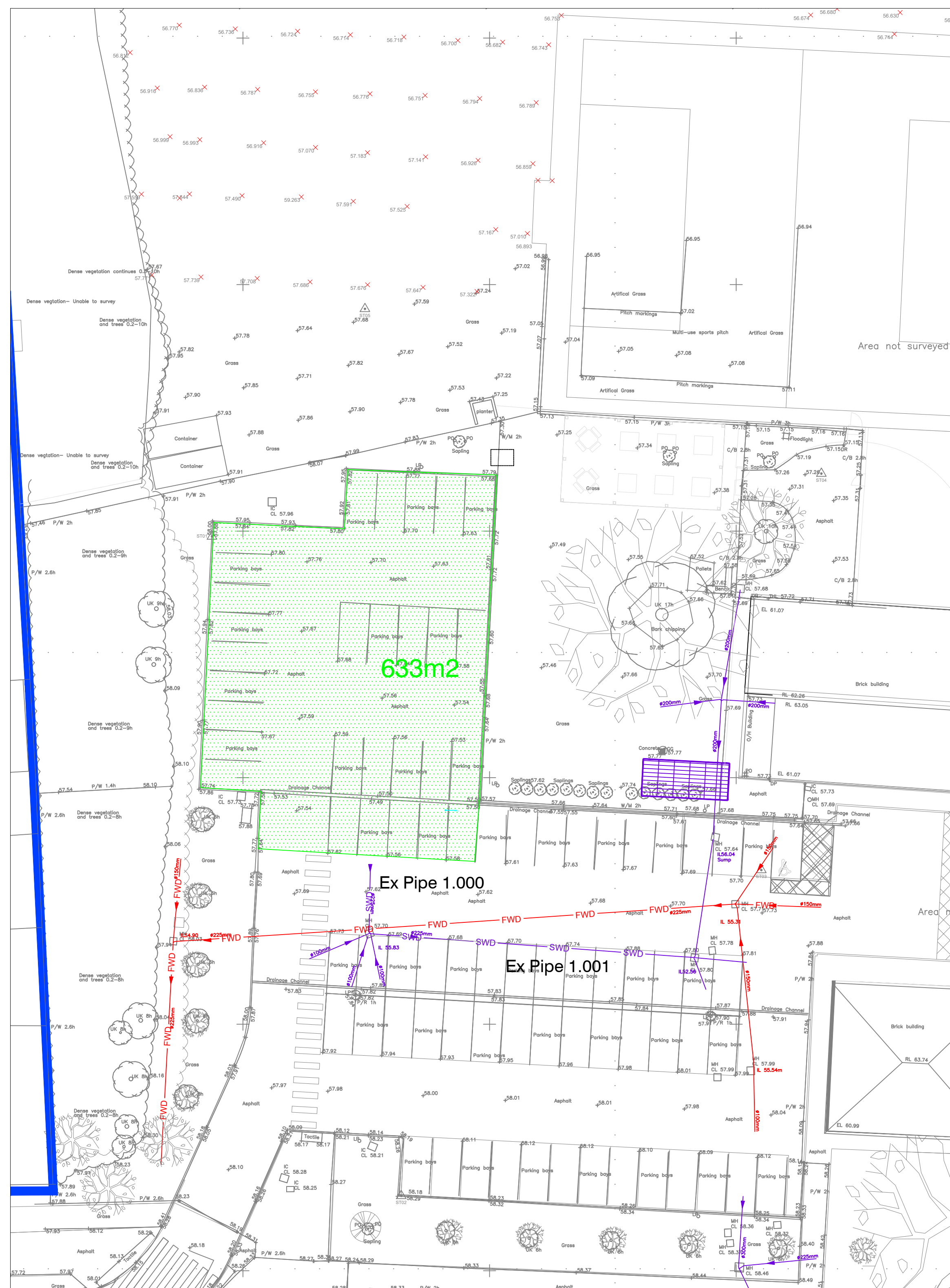
Existing Drained Impermeable Area
