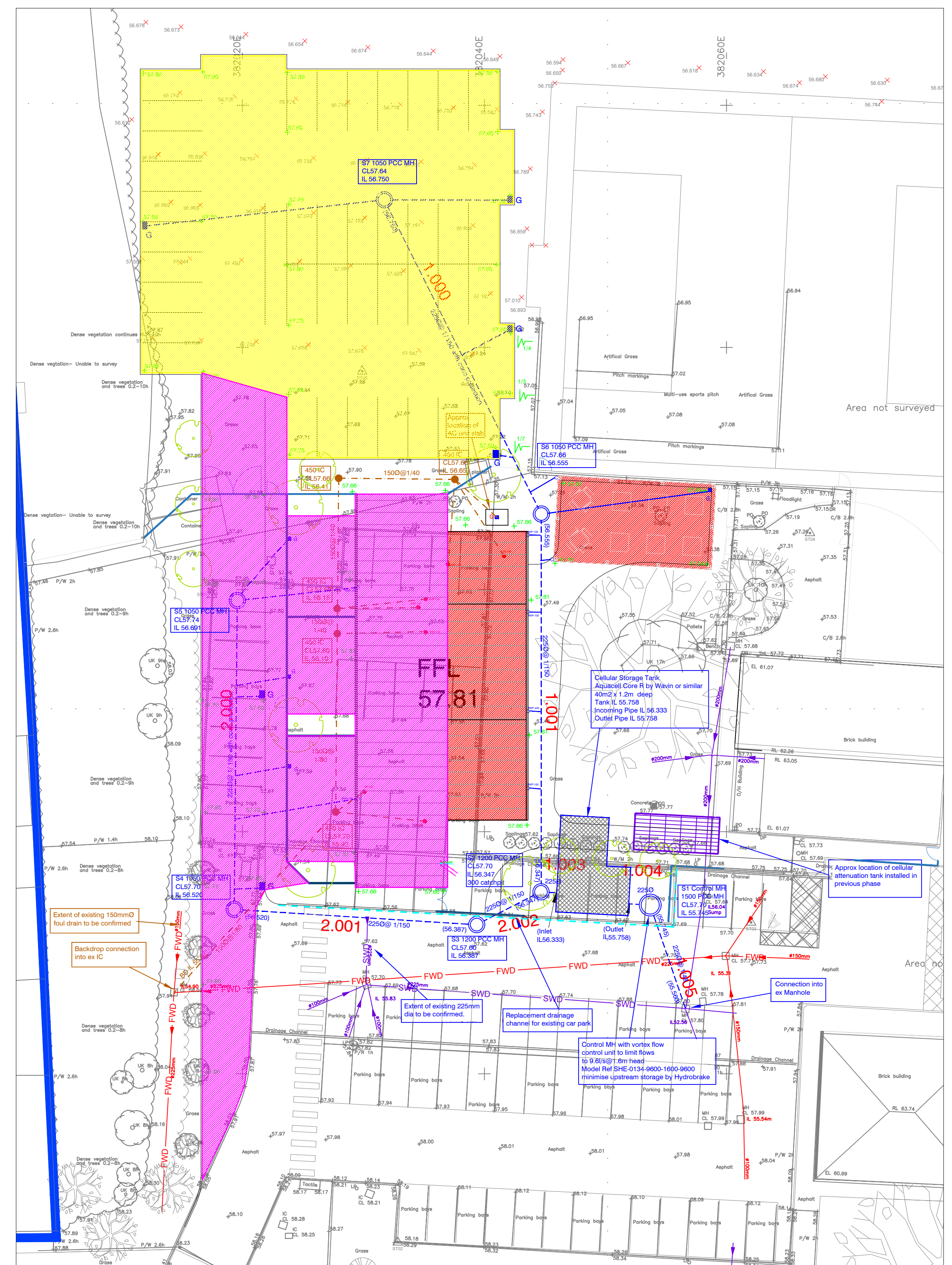
Proposed Contributing Area
