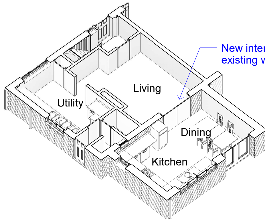
2 GF Plan - Proposed
