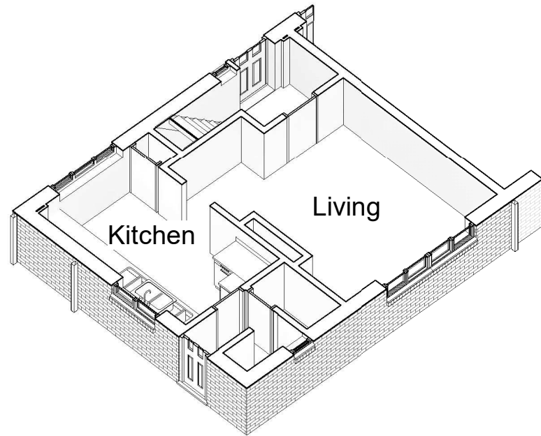
1 GF Plan - Existing
