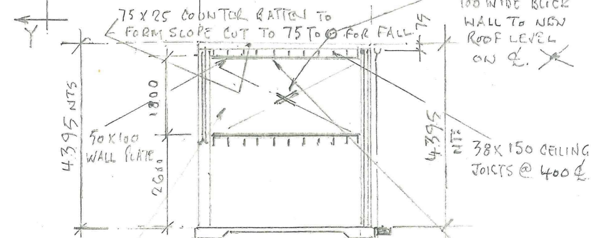
PROPOSED SECTION ON Y-Y
