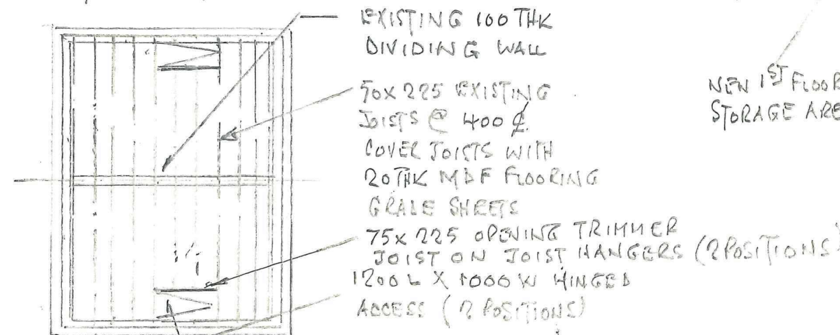
PROPOSED PLAN ON 1 ST FLOOR LEVEL A-A
