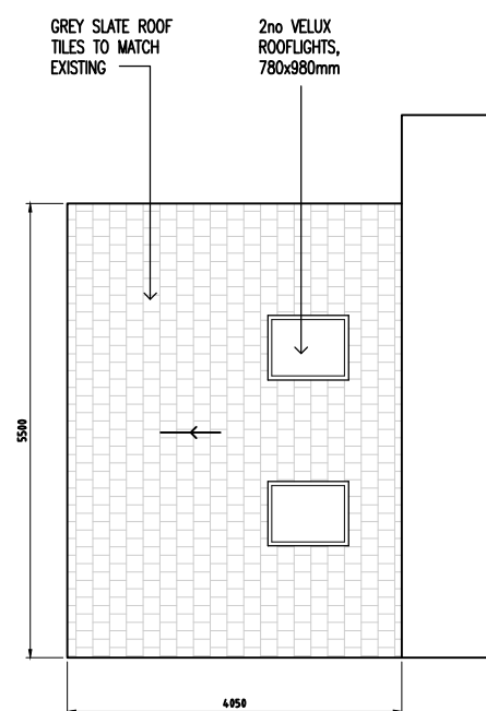
PROPOSED ROOF PLAN 1:100 @ A3
