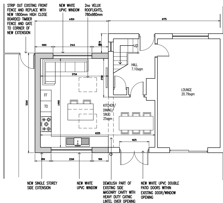
PROPOSED GROUND FLOOR PLAN 1:100 @ A3
