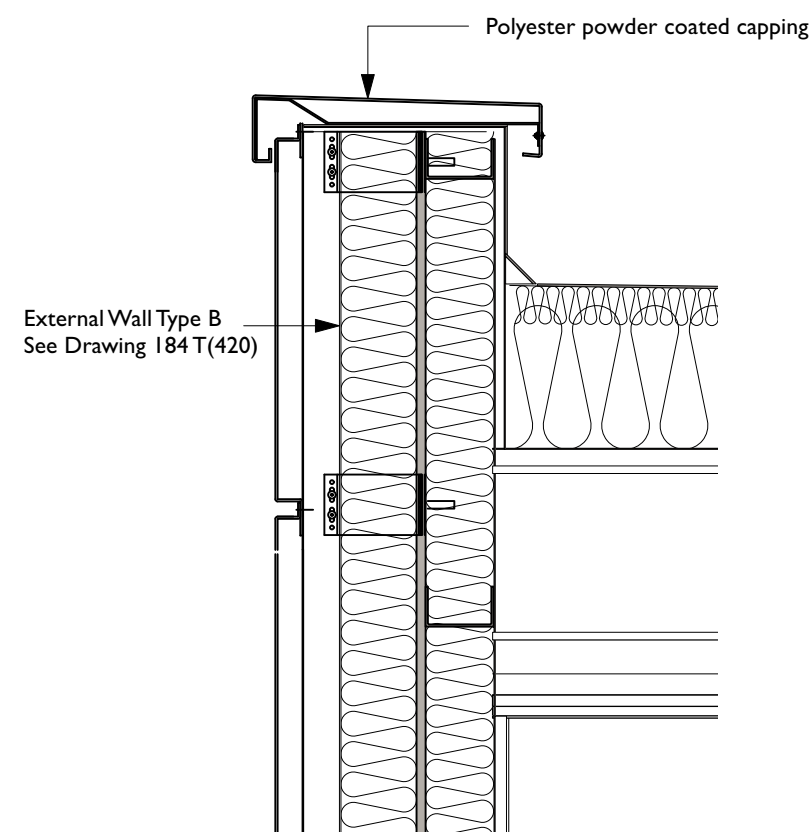
Roof Verge above Courtyard Scale: 1:10
