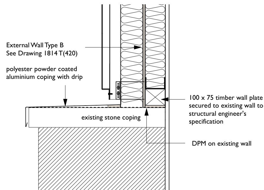
Base of New Wall over Courtyard Scale: 1:10
