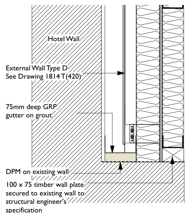
Base of New Wall Adjacent to Hotel Scale: 1:10
