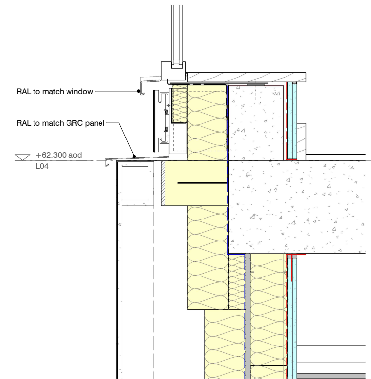
1 | Flashing Detail 1 : 10
