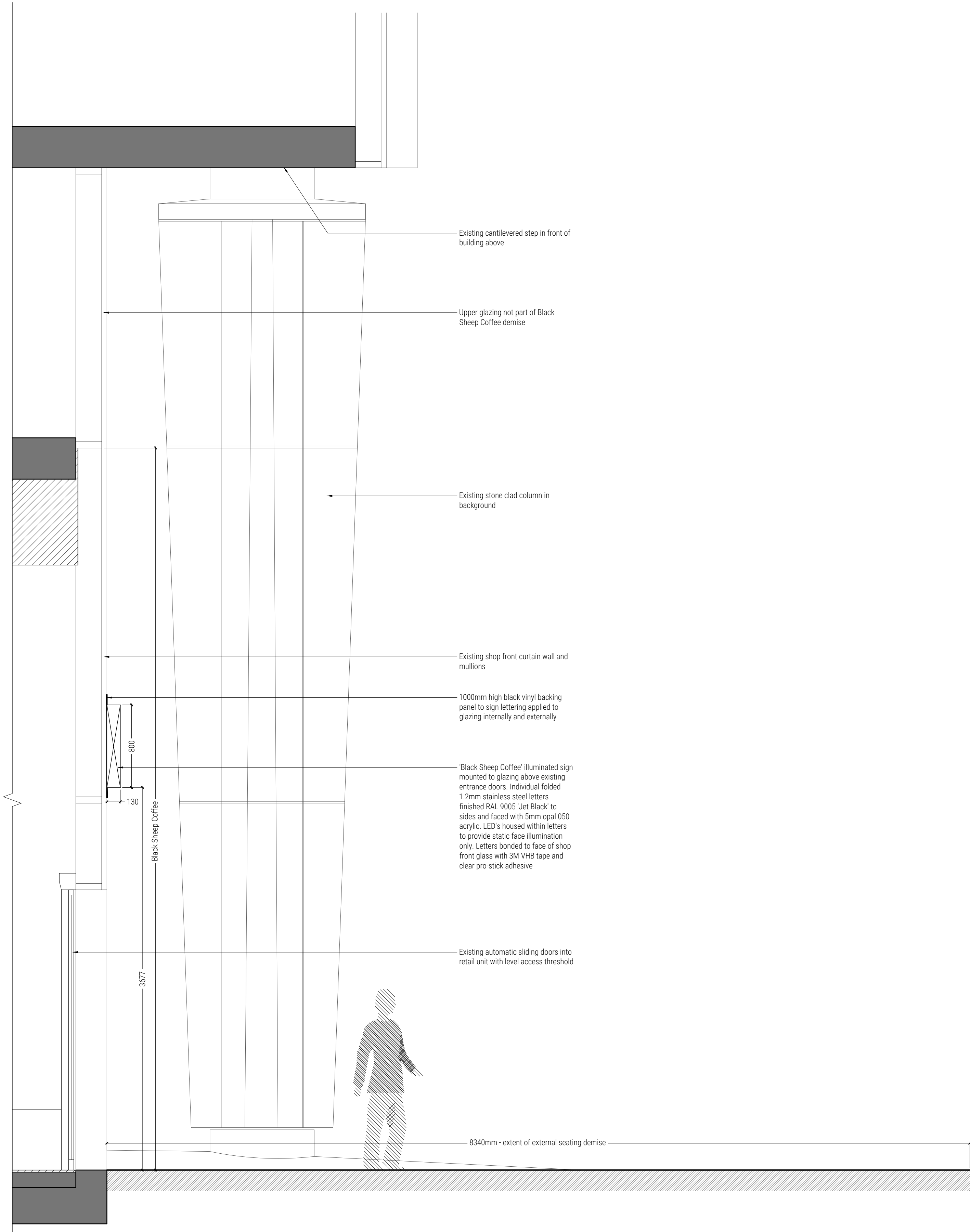
Section A: Typical Section Through Shop Front Section location as noted on drawing 9551-P-04
