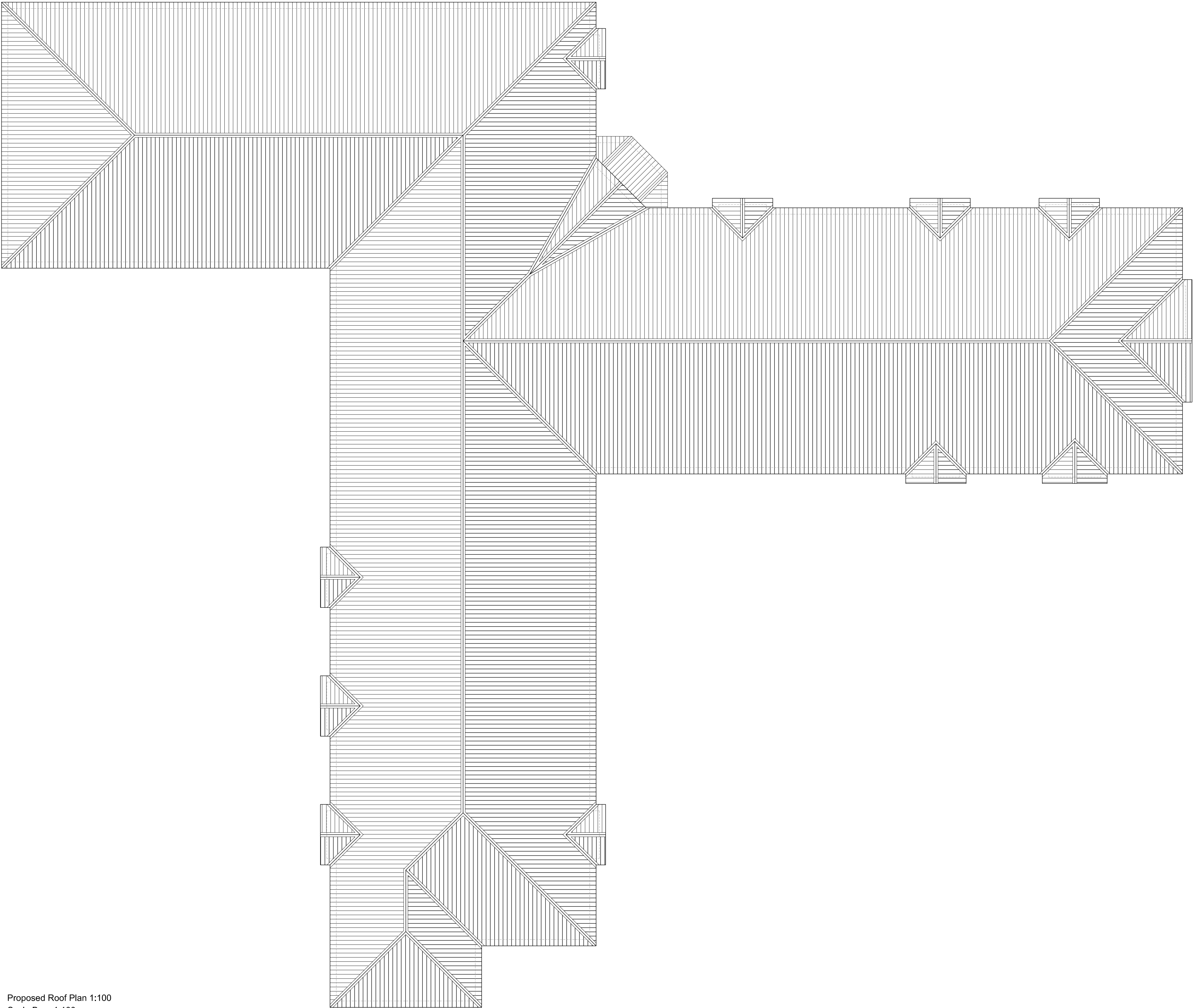
Proposed Roof Plan 1:100 Scale Bar 1:100 0 5 10m
