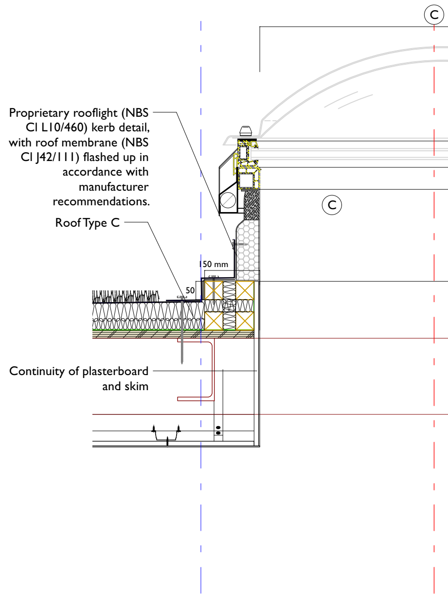
1 Rooflight Kerb Scale: 1:10
