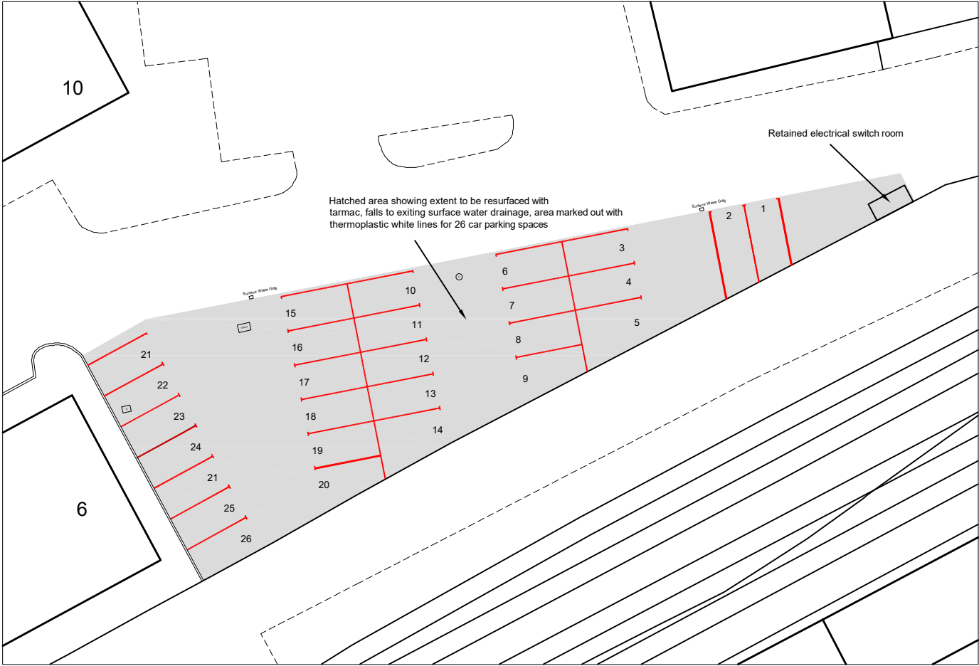
Proposed - Parking for 26 Vehicles (1:200)
