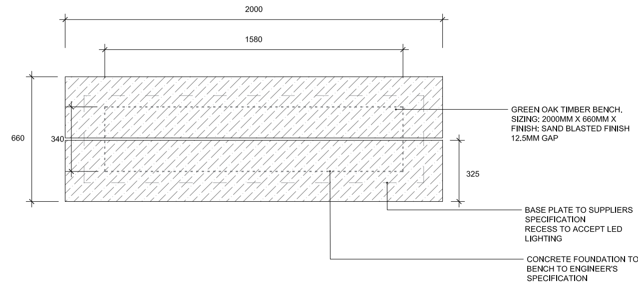
03C BRAMMHALL 1840 GREEN OAK TIMBER BENCH - CENTRAL SPACE PLAN SCALE 1:20
