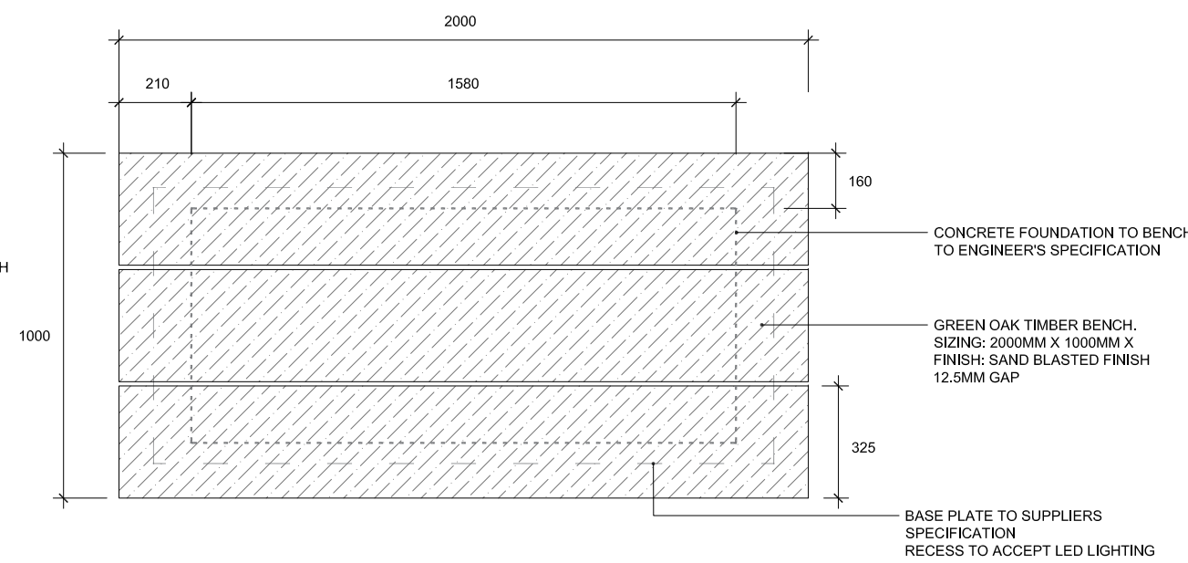
02C BRAMMHALL 1840 GREEN OAK TIMBER BENCH- CHORLTON SQUARE & CANAL EDGE PLAN SCALE 1:20
