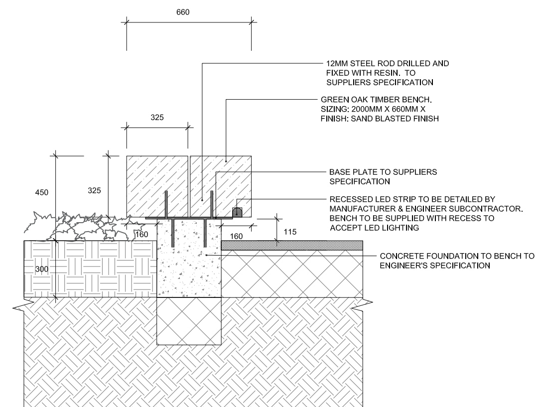
03A BRAMMHALL 1840 GREEN OAK TIMBER BENCH - CENTRAL SPACE SECTION SCALE 1:20
