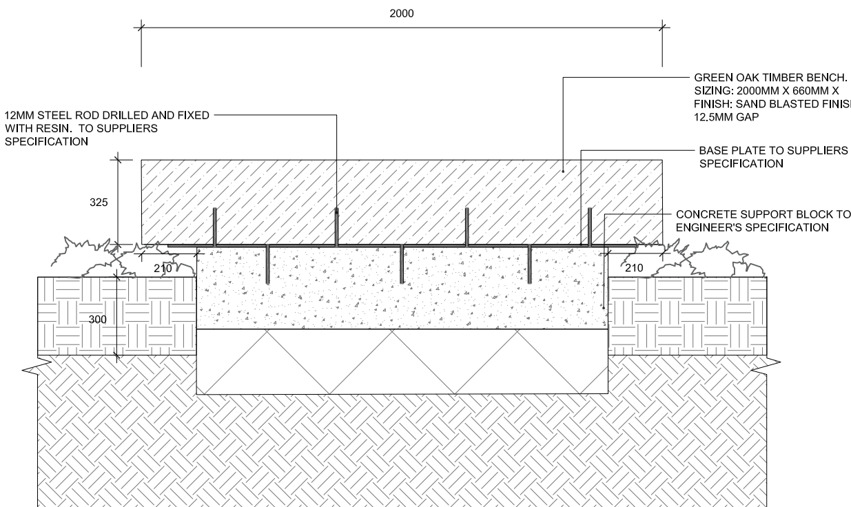
03B BRAMMHALL 1840 GREEN OAK TIMBER BENCH - CENTRAL SPACE SECTION SCALE 1:20
