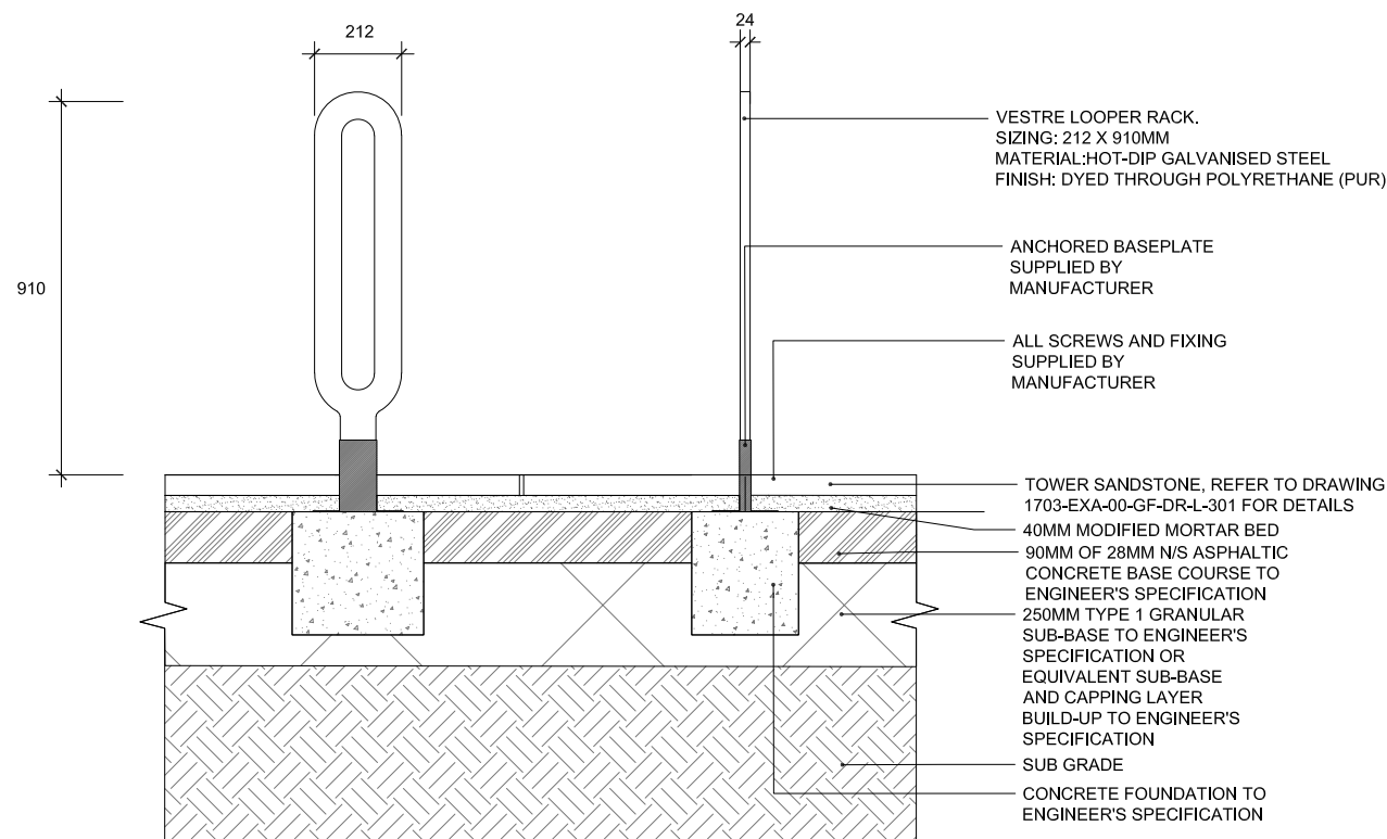
01A VESTRE LOOPER CYCLE RACK SECTION SCALE 1:20
