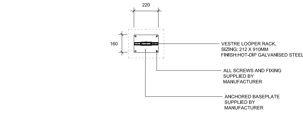
01B VESTRE LOOPER CYCLE RACK PLAN
