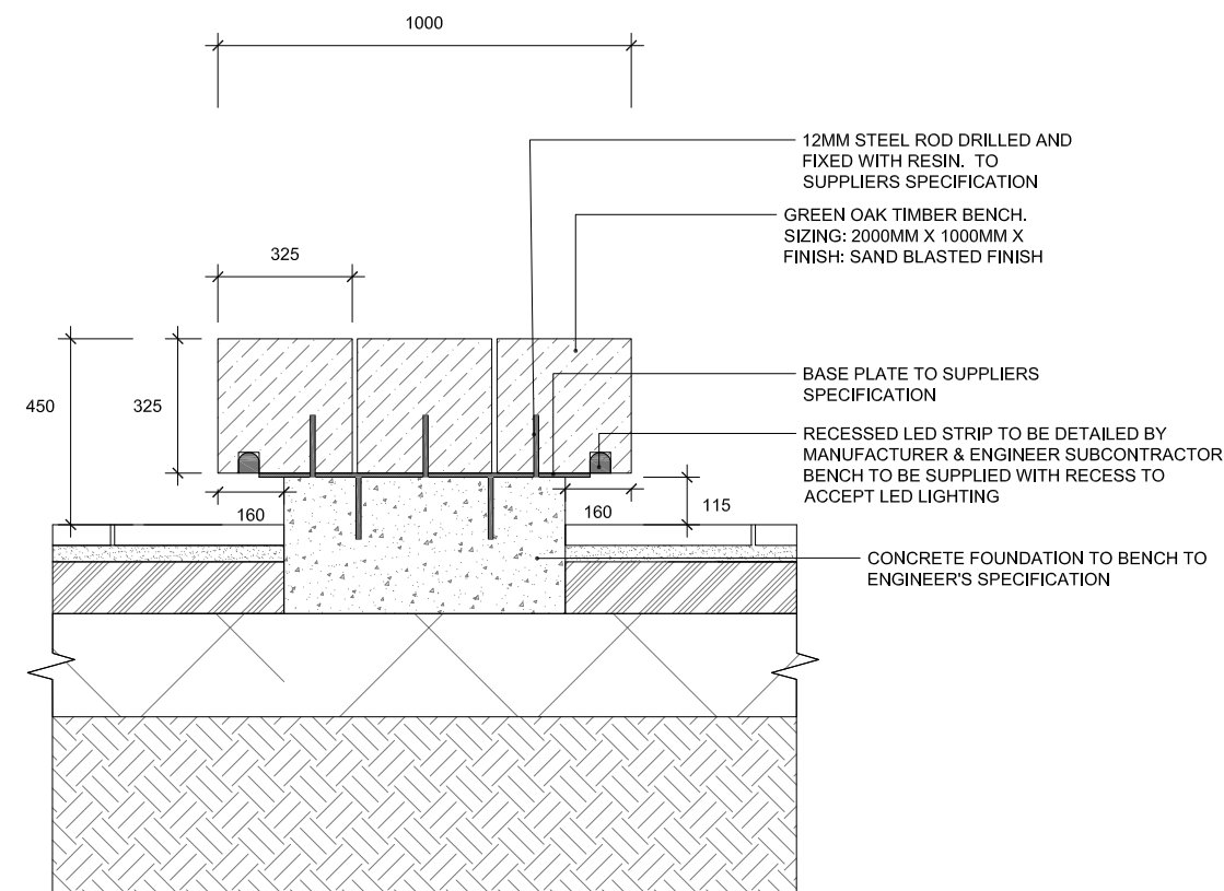
02A BRAMMHALL 1840 GREEN OAK TIMBER BENCH- CHORLTON SQUARE & CANAL EDGE SECTION SCALE 1:20
