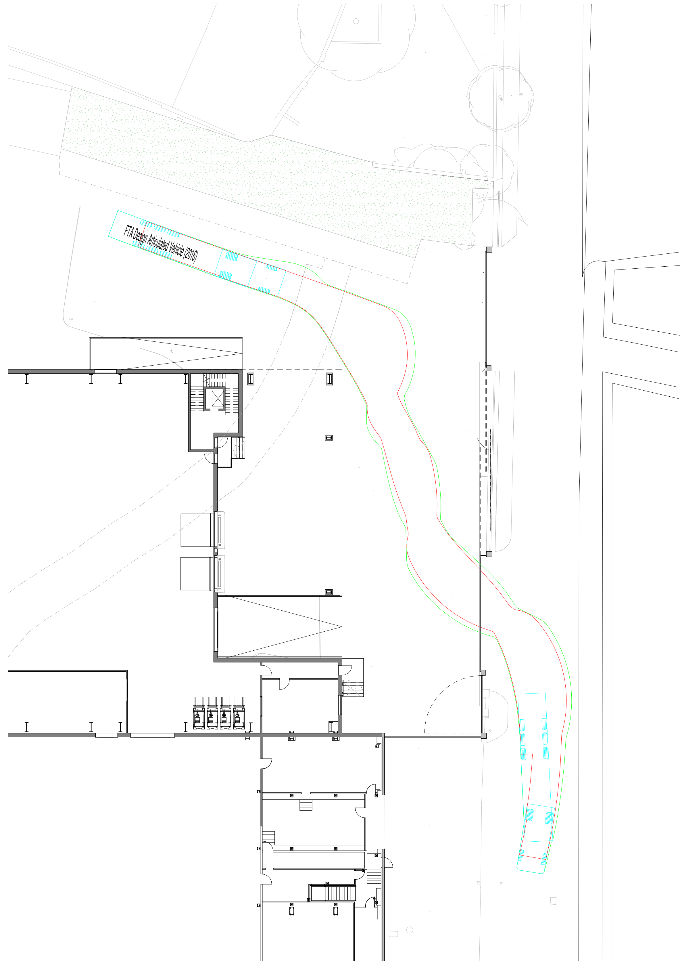
2 11-901 - HGV Vehicle Tracking Exit 1 : 200
