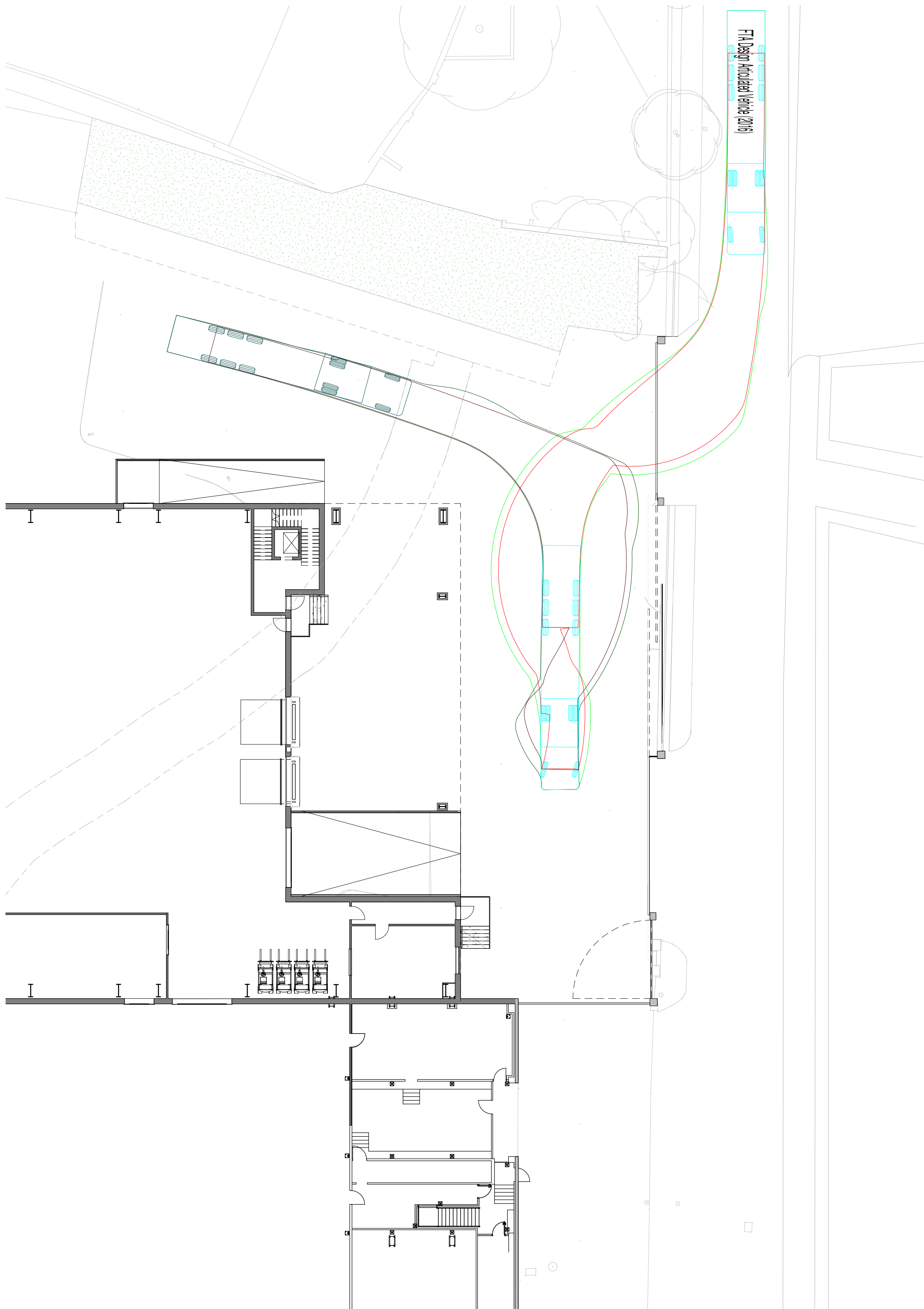
1 11-901 - HGV Vehicle Tracking Entrance 1 : 200
