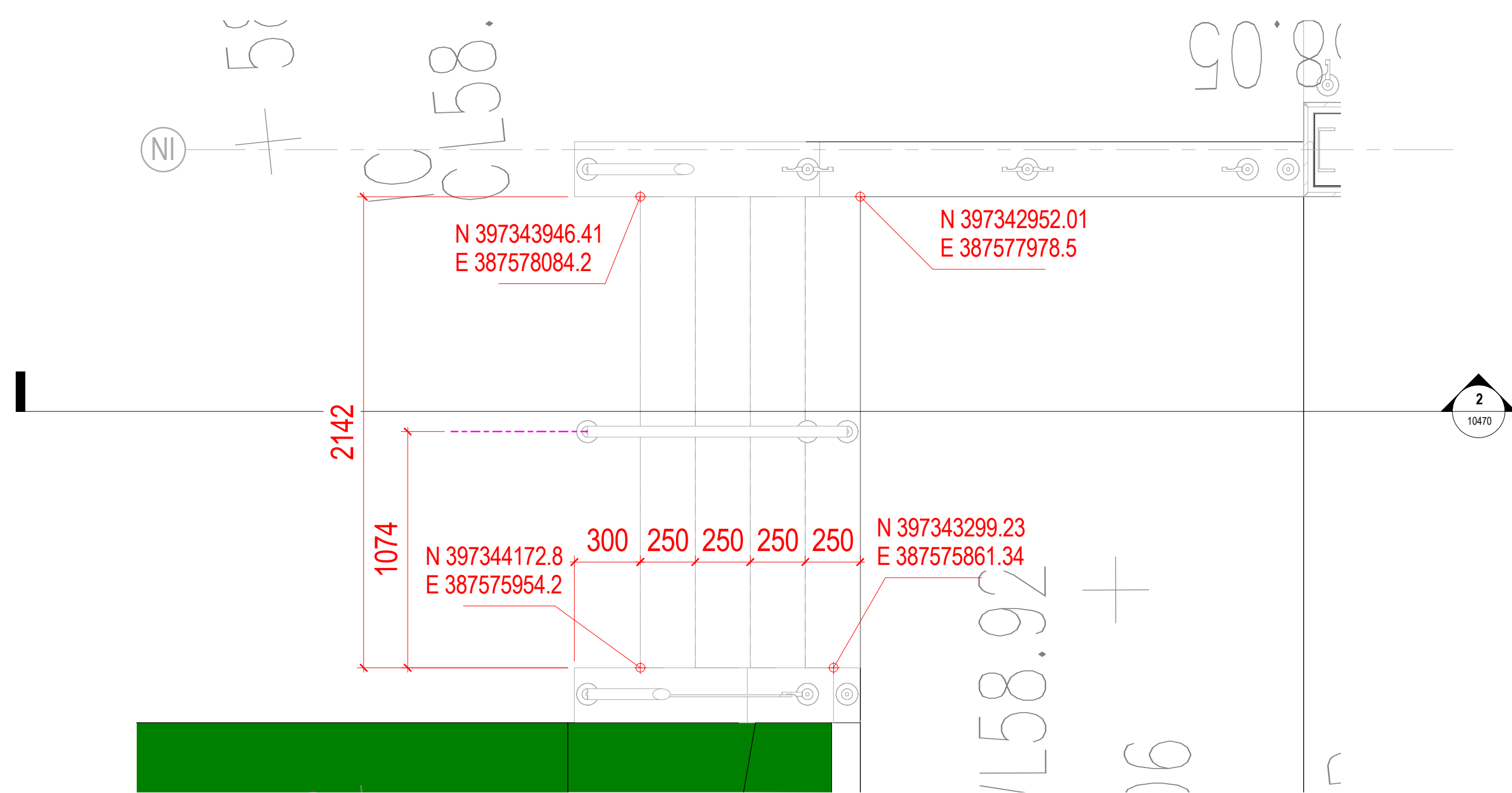
3 | PROPOSED EXTERNAL STAIRCASE SETTING OUT PLAN
