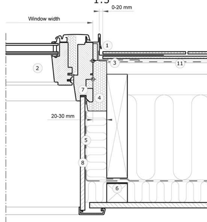
Section B-B 1:5
