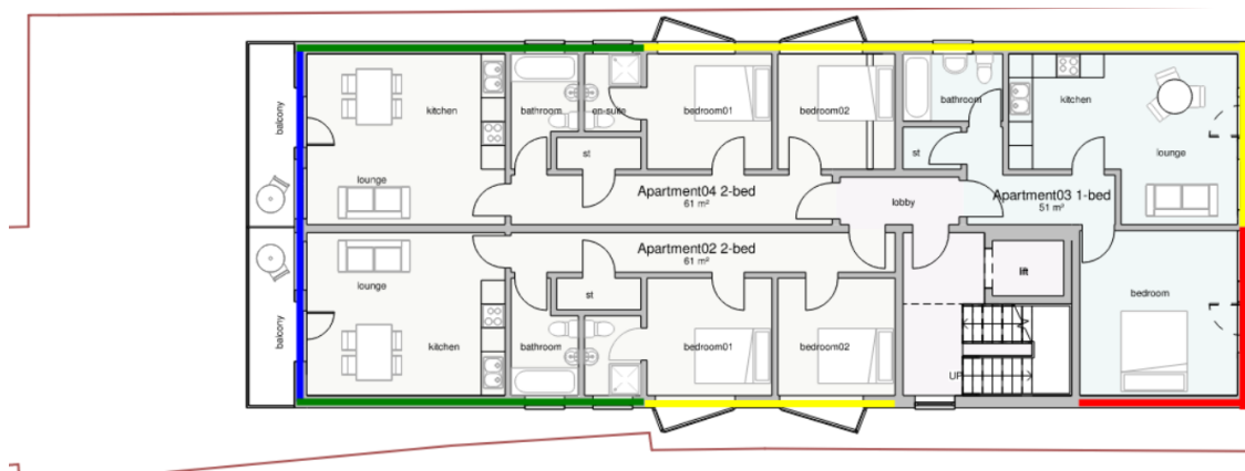
Figure 7 Levels 1, 2, 3, 4 – recommended minimum facade sound insulation performance
