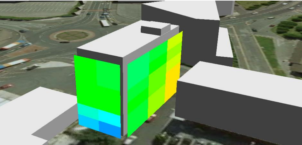
Figure 3 Image from 3D noise model – Daytime time noise levels West view
