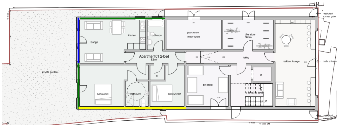
Figure 6 Ground floor level – recommended minimum facade sound insulation performance
