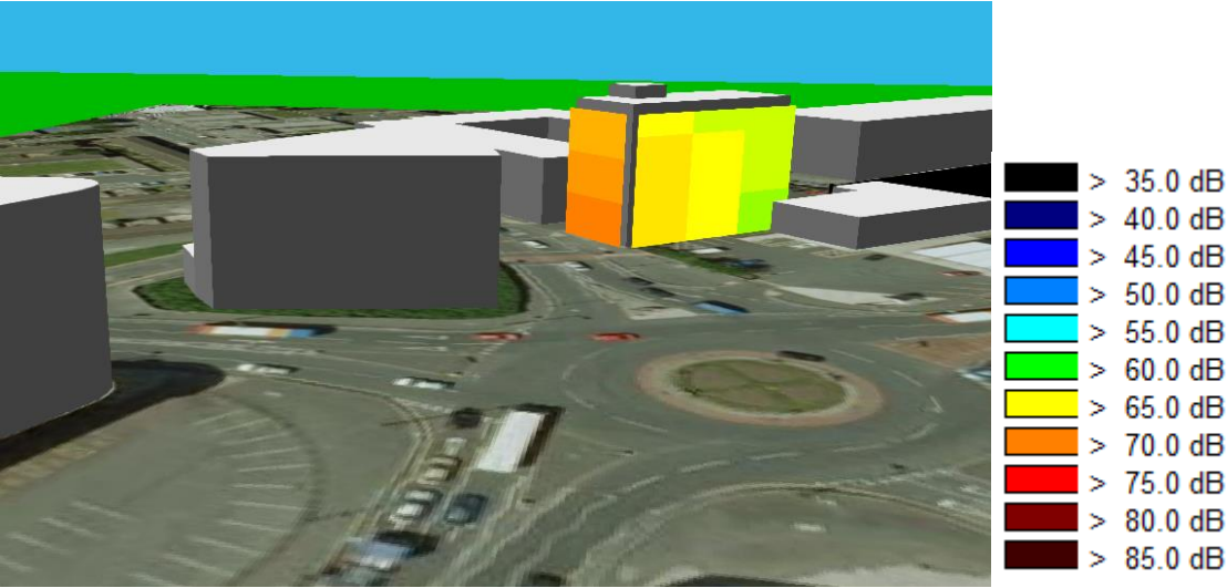
Figure 2 Image from 3D noise model – Daytime noise levels East view
