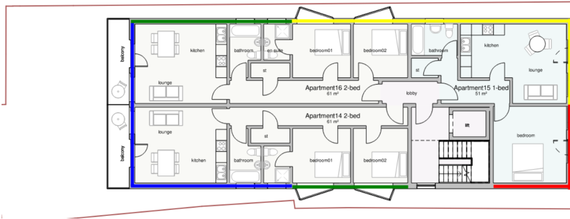
Figure 8 Level 5 – recommended minimum facade sound insulation performance
