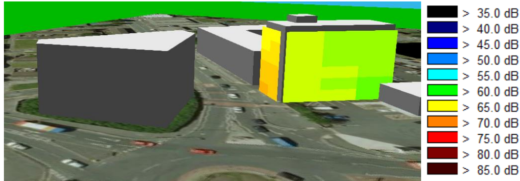
Figure 4 Image from 3D noise model – Night-time noise levels – East view
