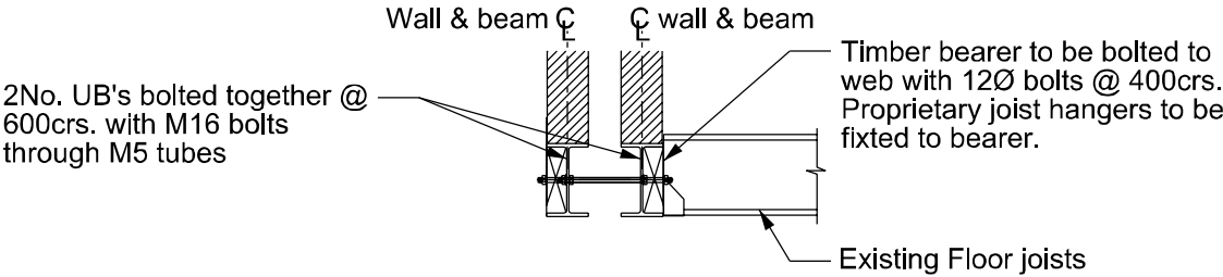
Cavity Wall Beam Support Detail 1:20
