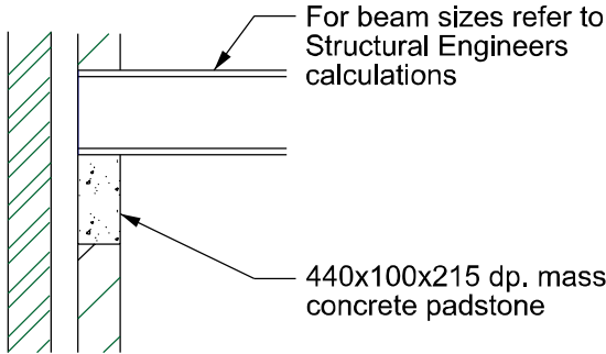
Section Thro' Typical Beam Bearing Detail 1:20
