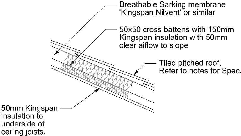
Sloping Roof Insulation Detail 1:25
