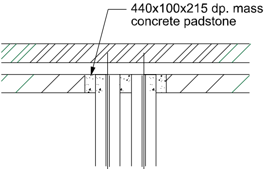
Plan on Typical Beam Bearing Detail 1:20
