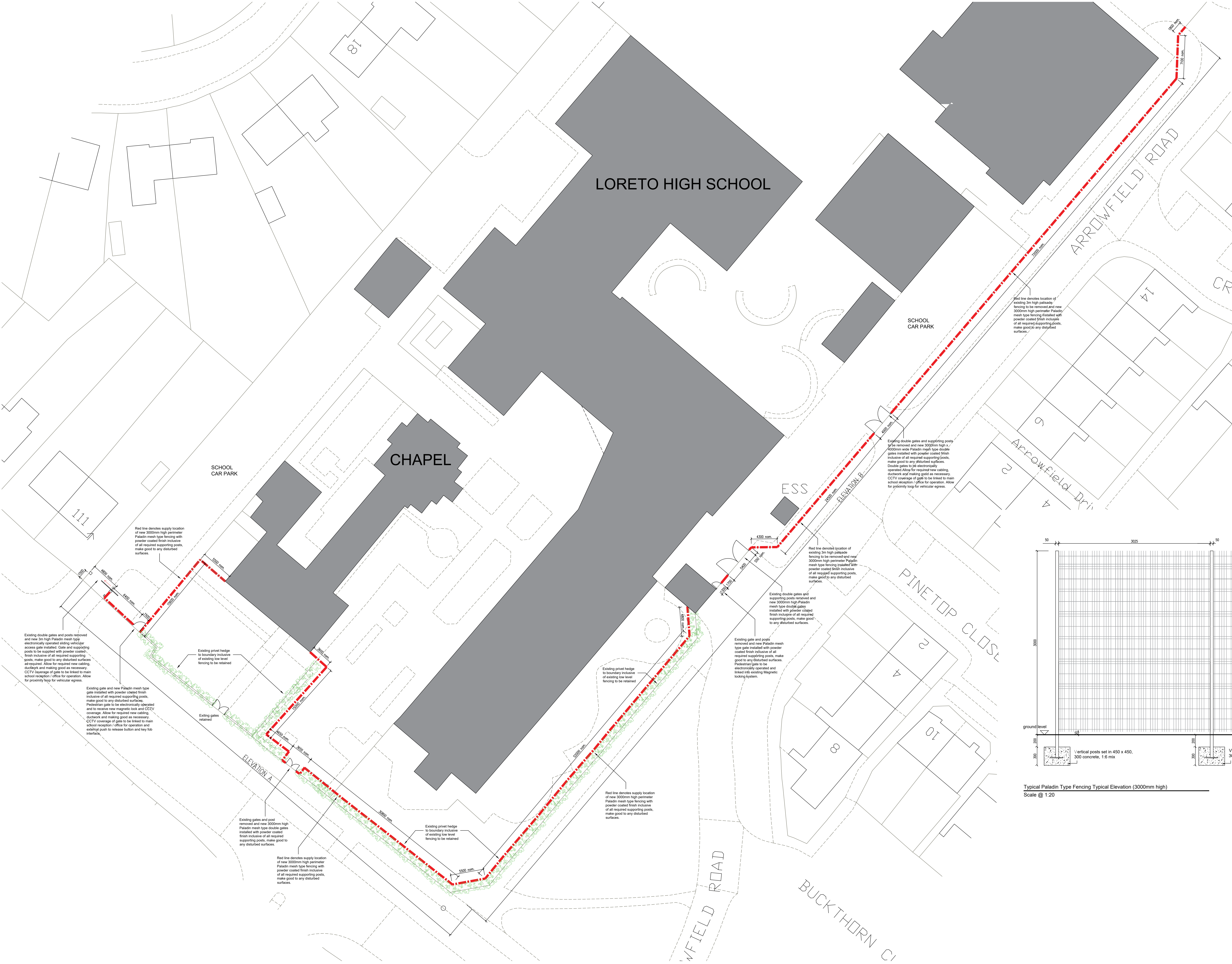
Proposed Part Site / Block Plan as Proposed Scale @ 1:200
