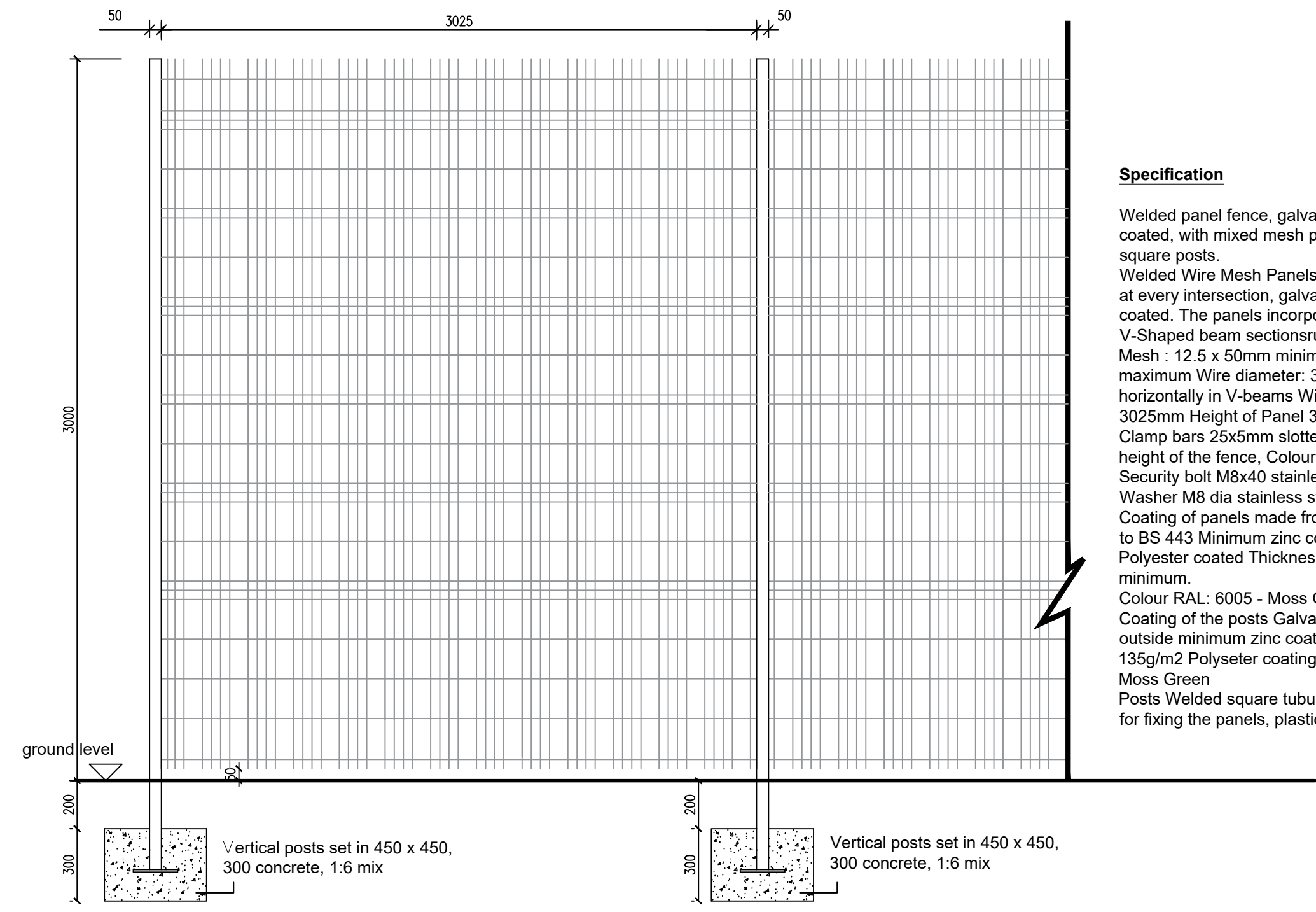
Typical Paladin Type Fencing Typical Elevation (3000mm high) Scale @ 1:20
