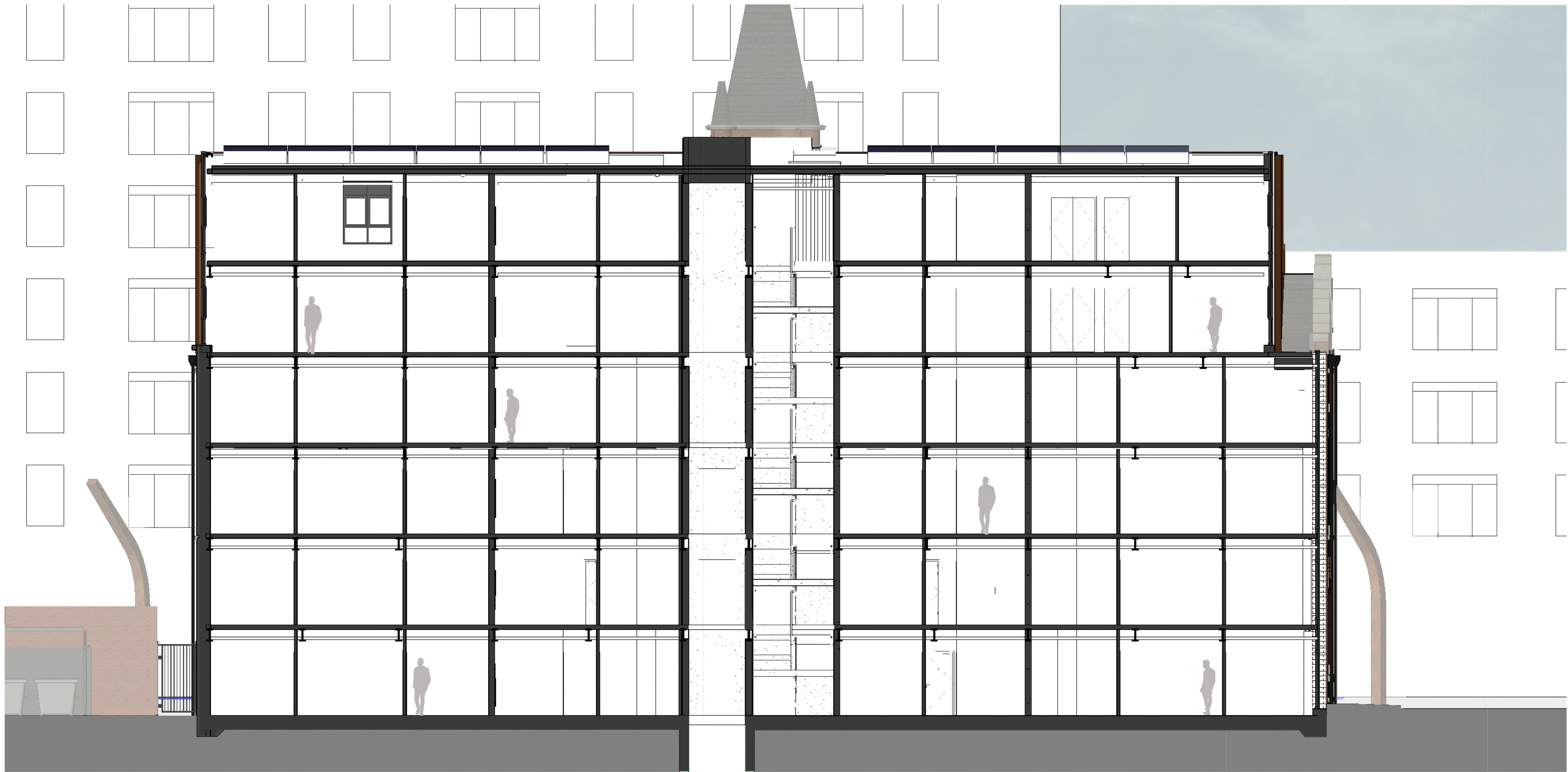
Long Section E - Proposed 1:100
