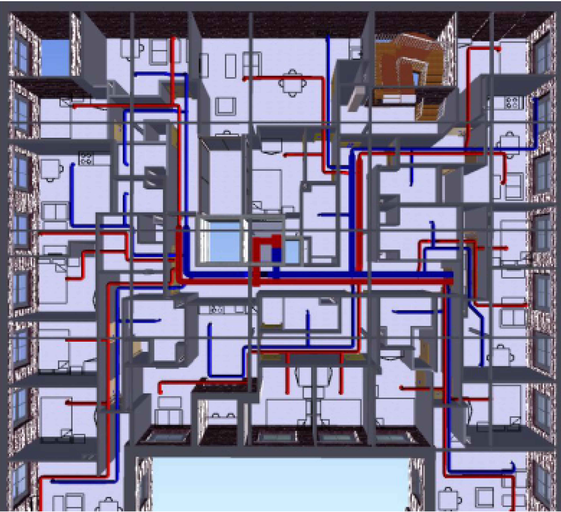
REVIT MODEL SCREENSHOT SHOWING INDICATIVE DUCTWORK ON EACH FLOOR (NTS)
