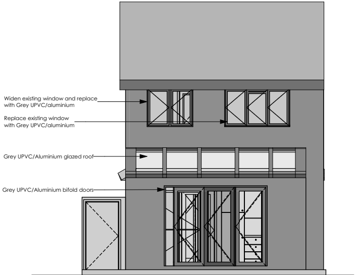
North Elevation 1:100
