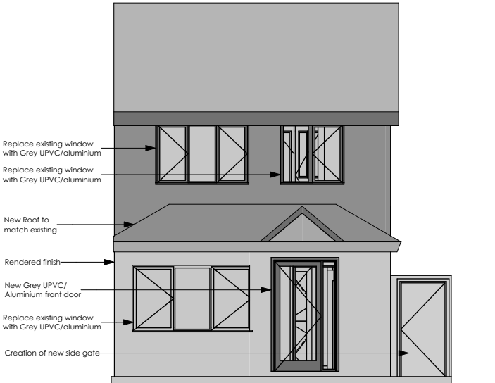
South Elevation 1:100
