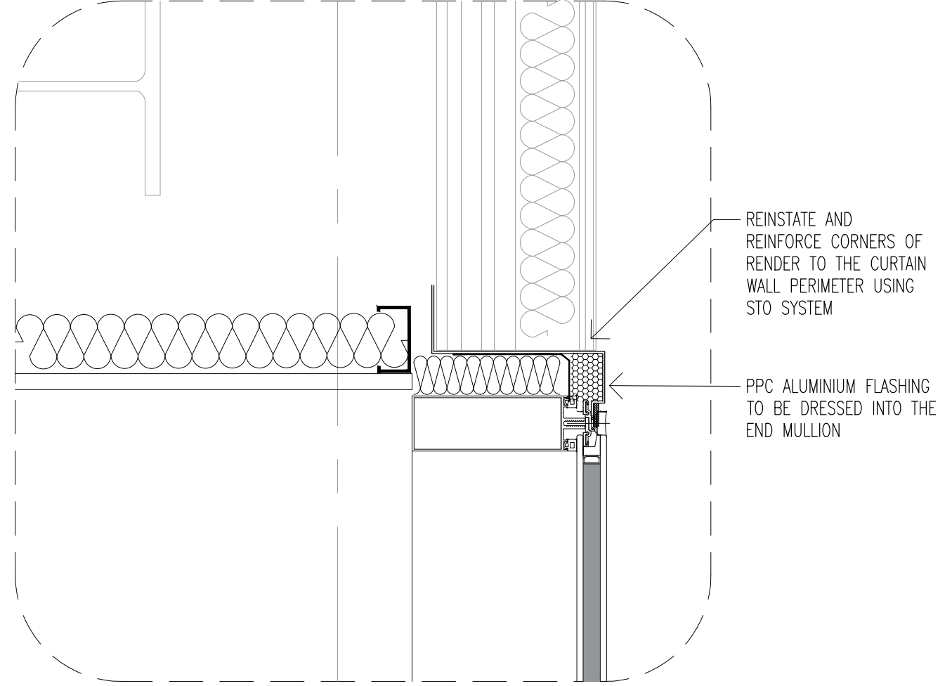
CURTAIN WALL JAMB DETAIL 1:5@A1
