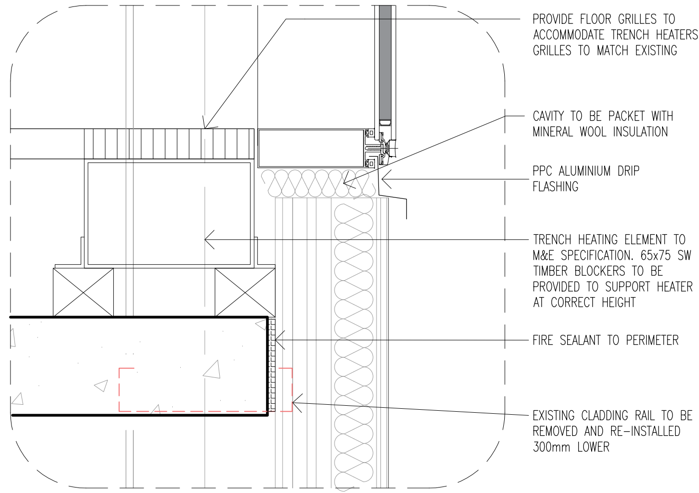
DETAIL 2 1:5 @ A1
