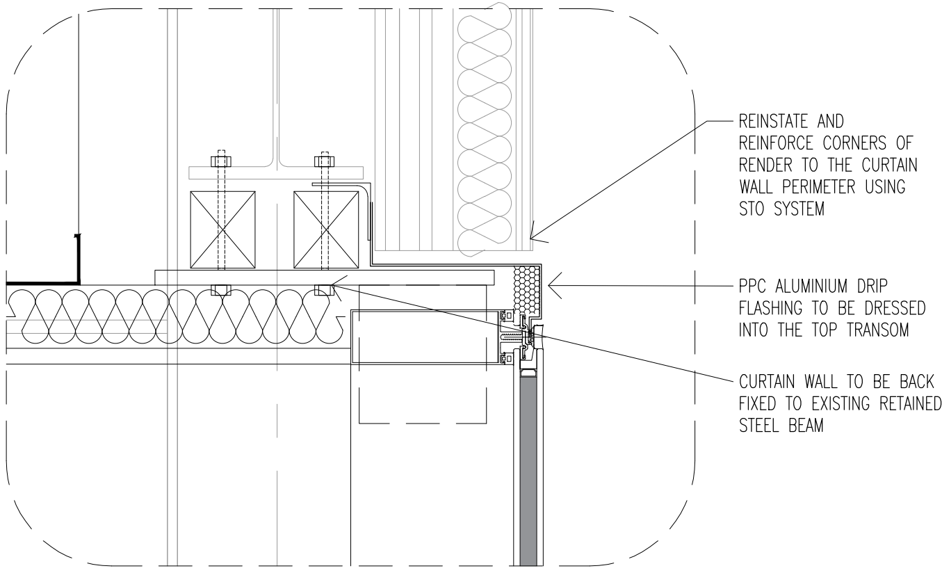
DETAIL 1 1:5 @ A1
