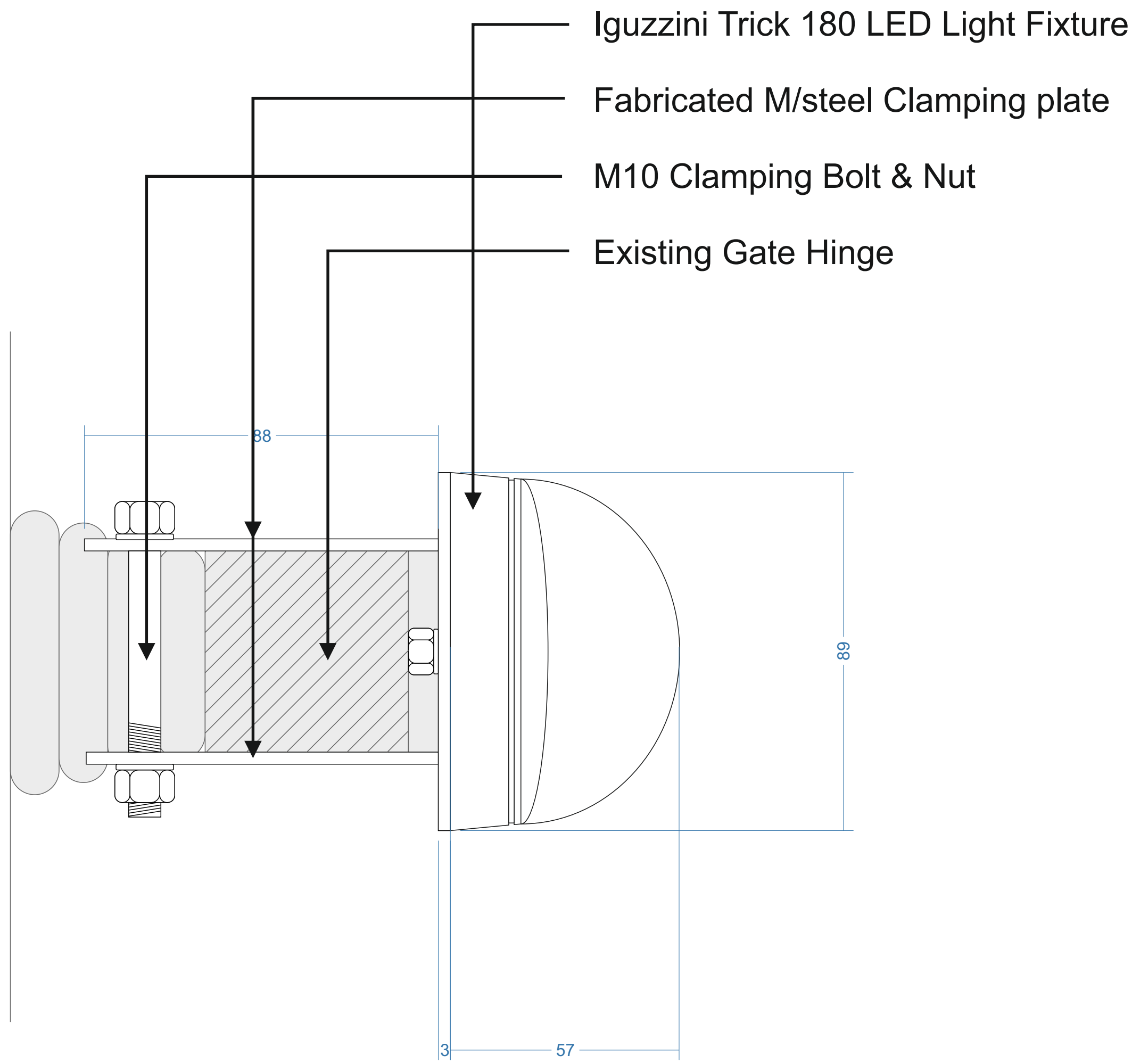
Hinge Mount Section A-A Scale 1:1 @ A0
