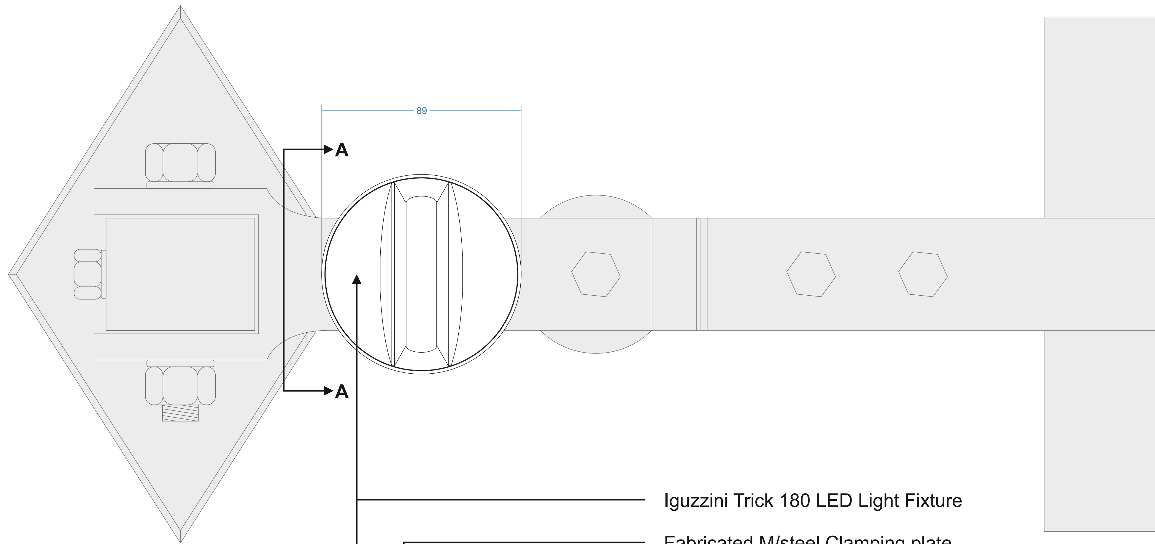
Hinge Mount Front View Scale 1:1 @ A0
