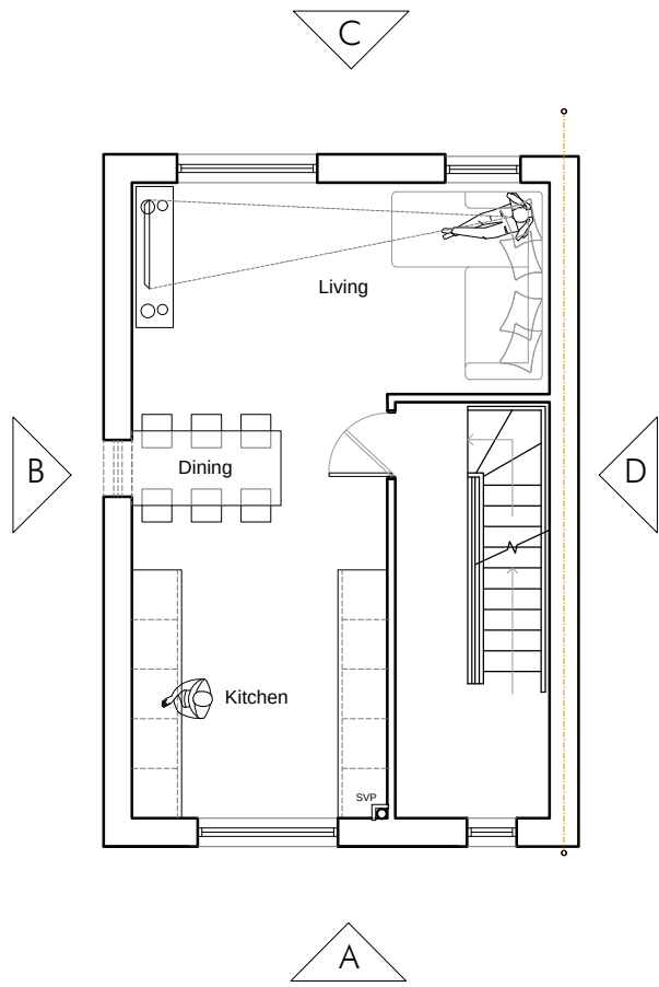
First Floor 38m 2 /418ft 2
