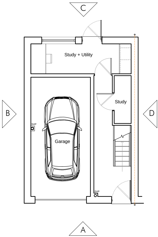
Ground Floor - ex Garage 19m 2 /206ft 2
