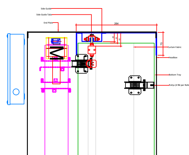
03/001 Plan Section Of Headbox End SCALE 1 : 8 @ A3
