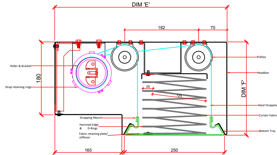
02/001 Section Through Headbox SCALE 1 : 5 @ A3
