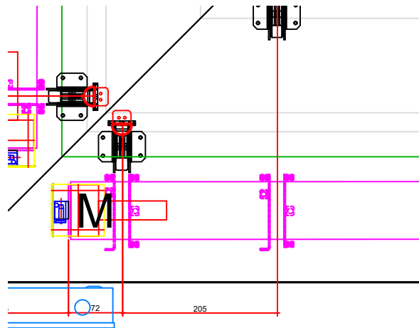
04/001 Plan Section Of Headbox Corner SCALE 1 : 10 @ A3
