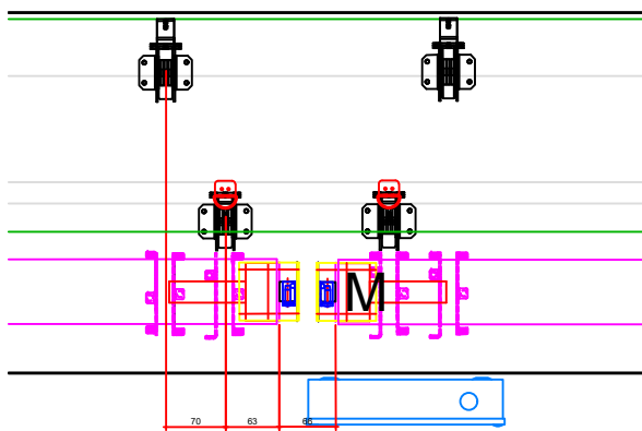
05/001 Plan Section Of Roller Separation SCALE 1 : 10 @ A3
