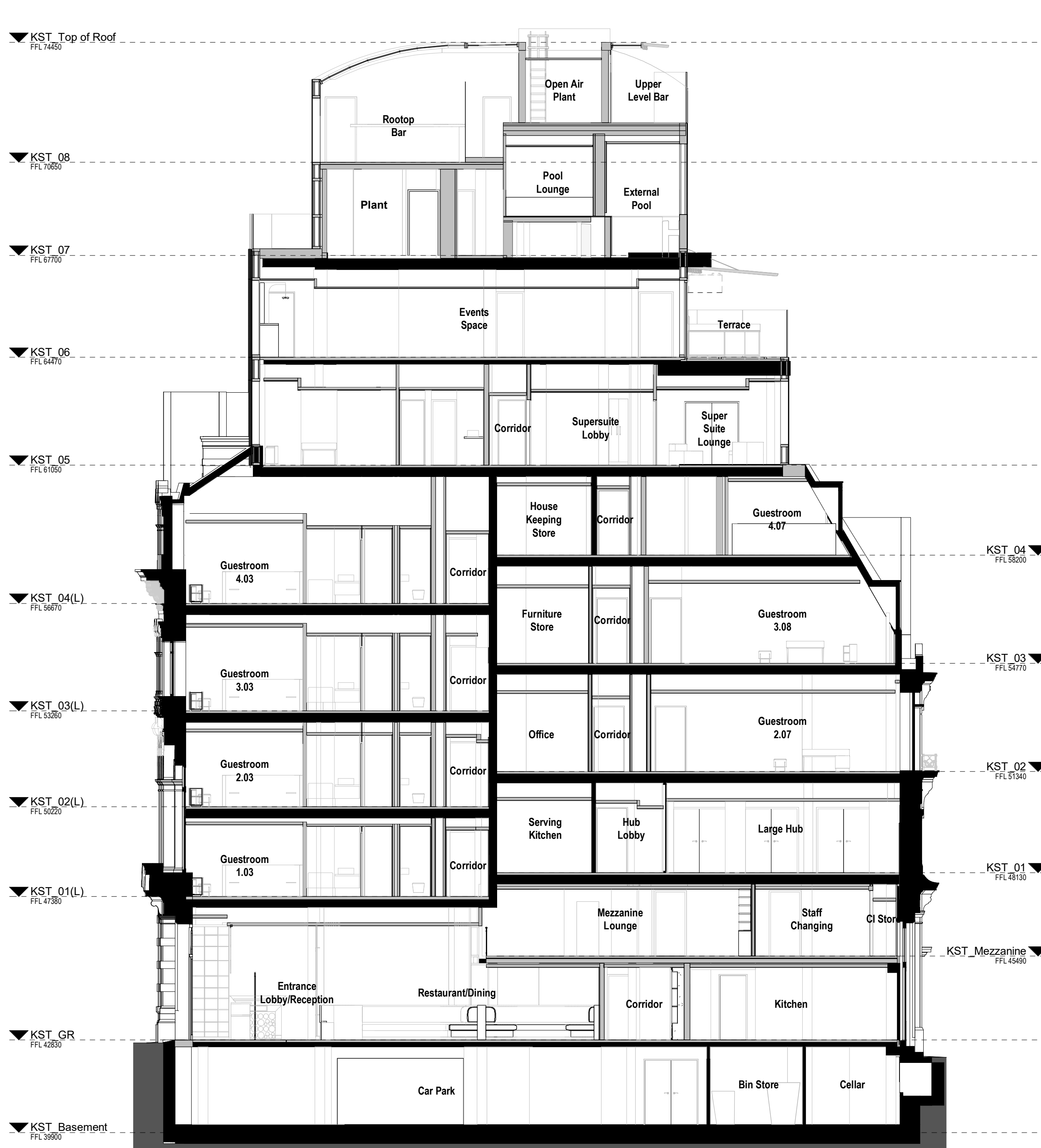
B Proposed Section BB 1: 100
