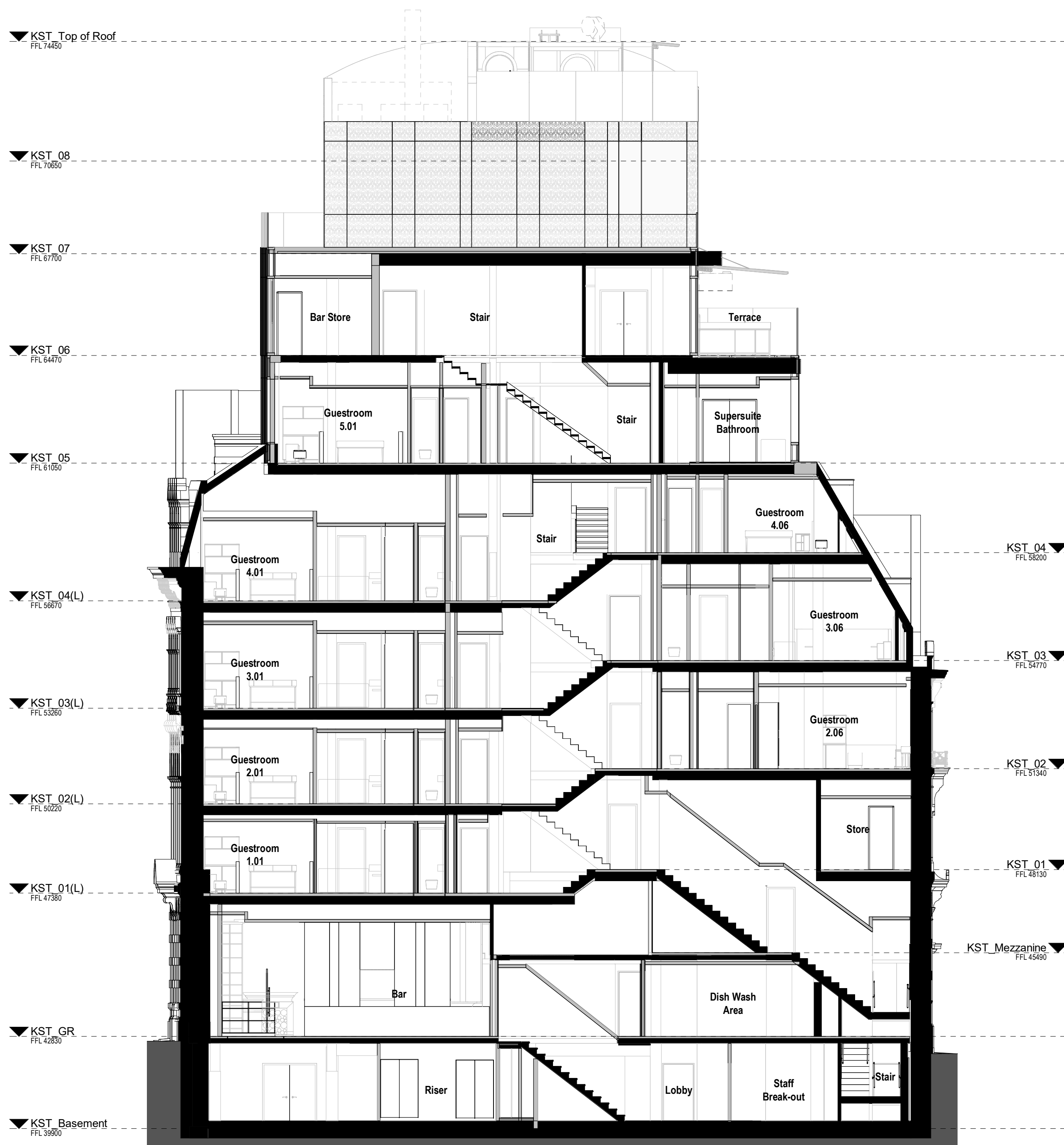
A Proposed Section AA 1: 100
