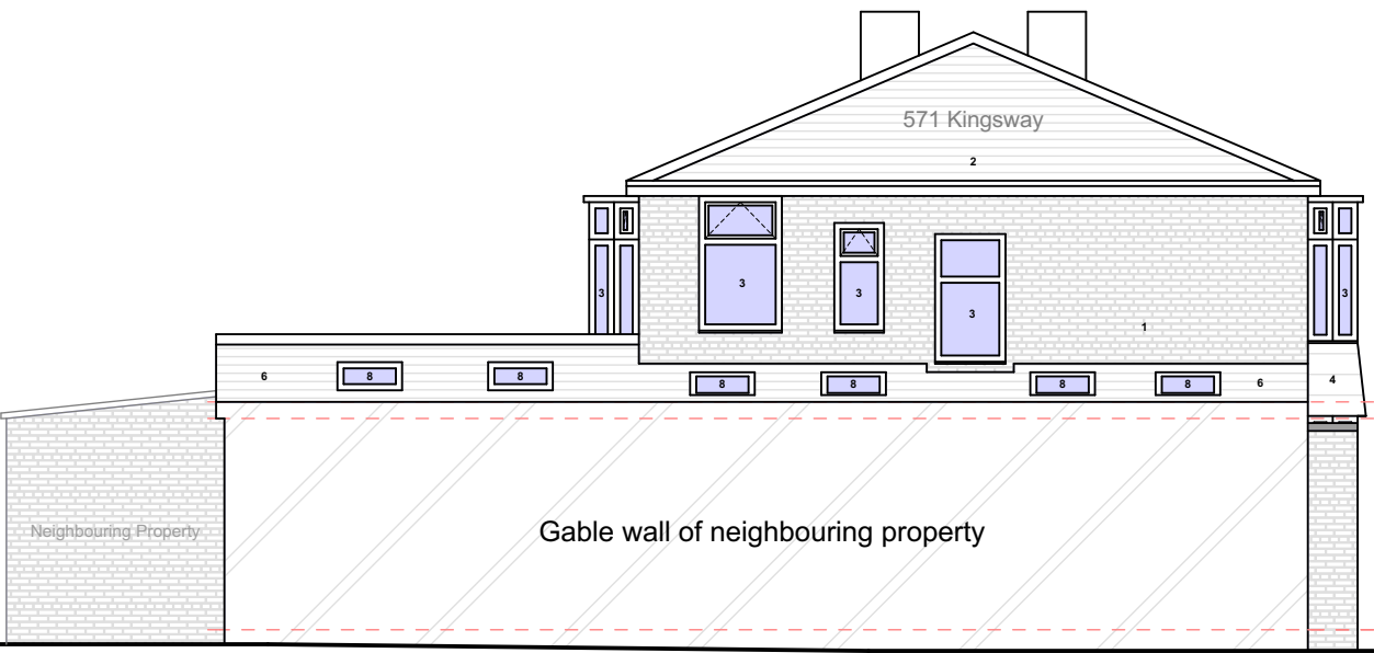
PROPOSED GA SIDE ELEVATION 1 (571 KINGSWAY)
