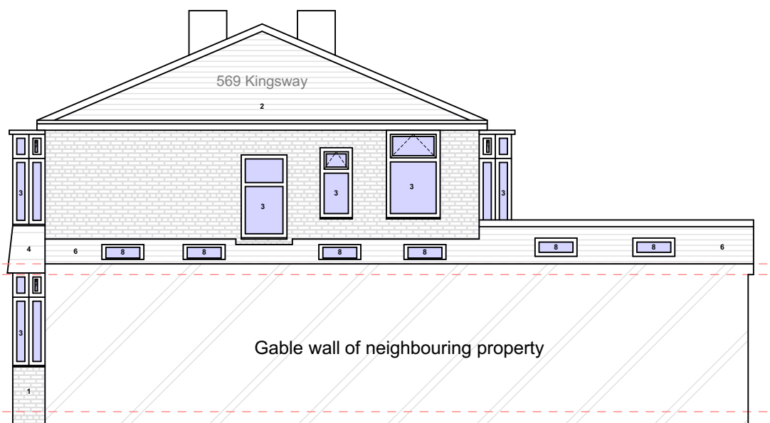
PROPOSED GA SIDE ELEVATION 1 (569 KINGSWAY)
