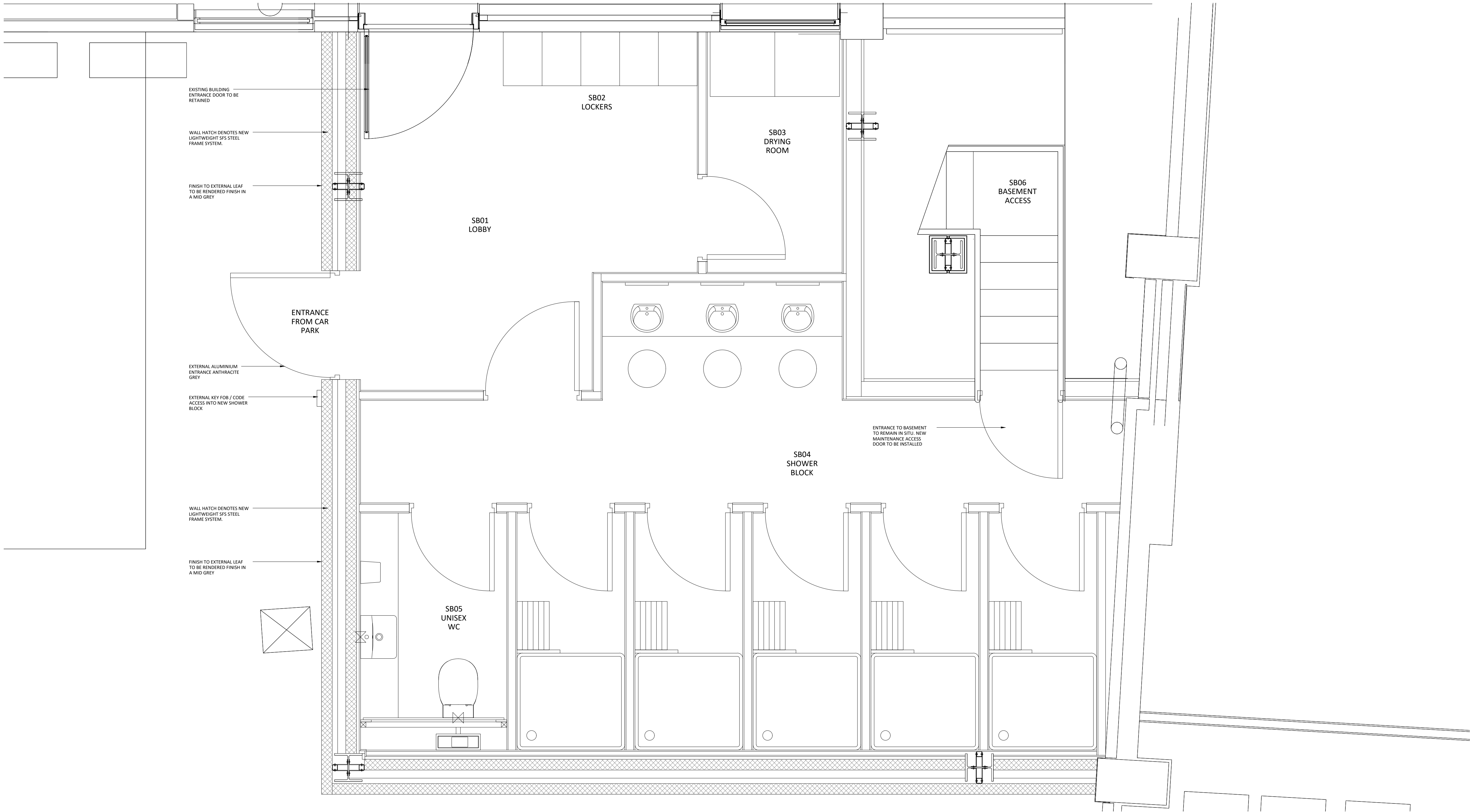
01 100 PROPOSED SHOWER FACILITY PLAN SCALE - 1:20@A1 PLAN
