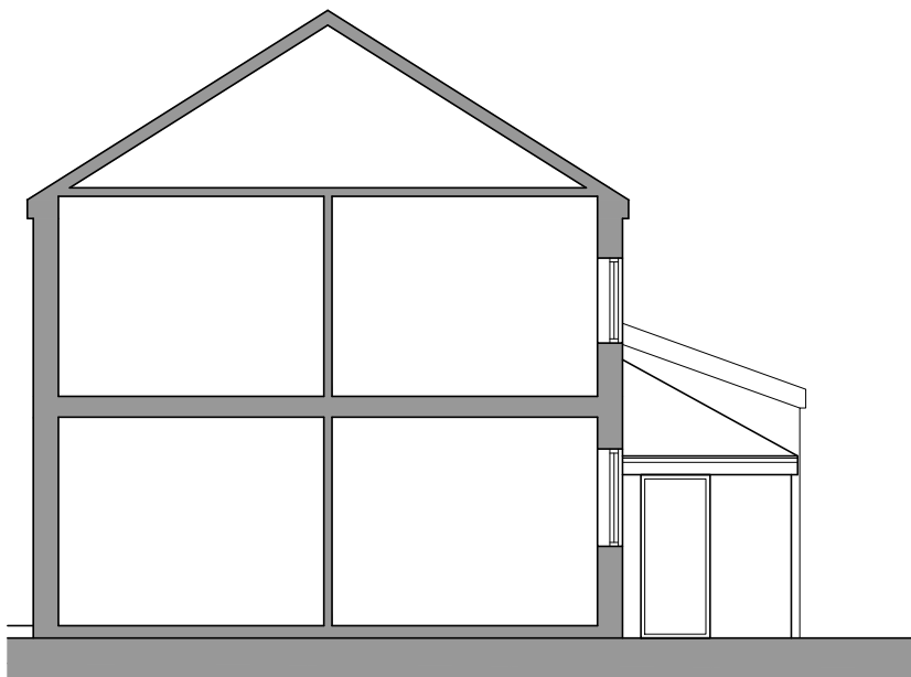
South East Facing Side Elevation
