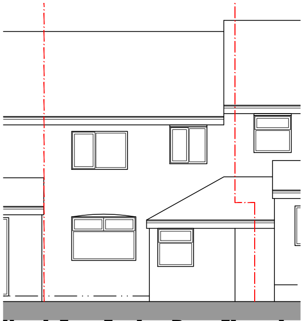
North East Facing Rear Elevation
