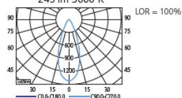
HARM G1 TRANSPARENT 245 lm 3000 K
