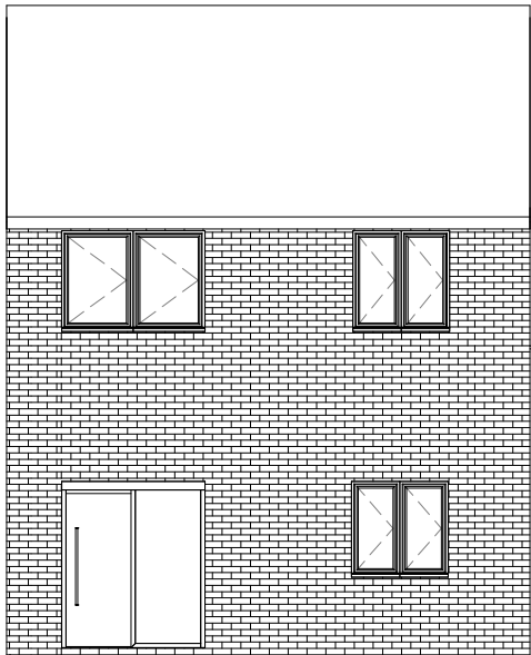
3 Rear Existing 1 : 100
