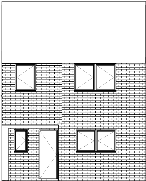
1 Front Existing 1 : 100
