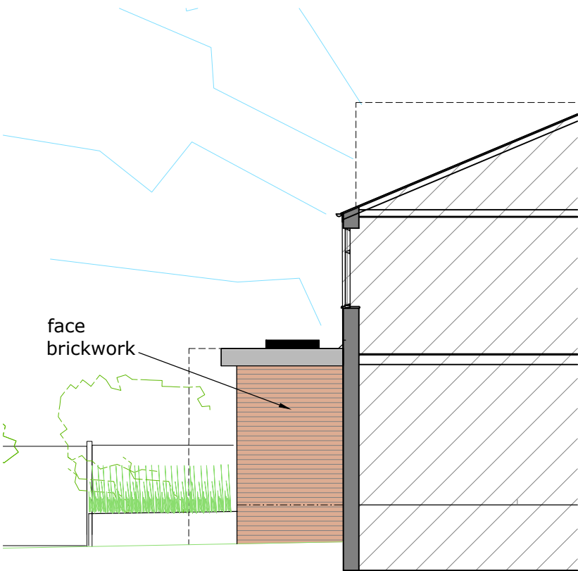
NORTH ELEVATION
