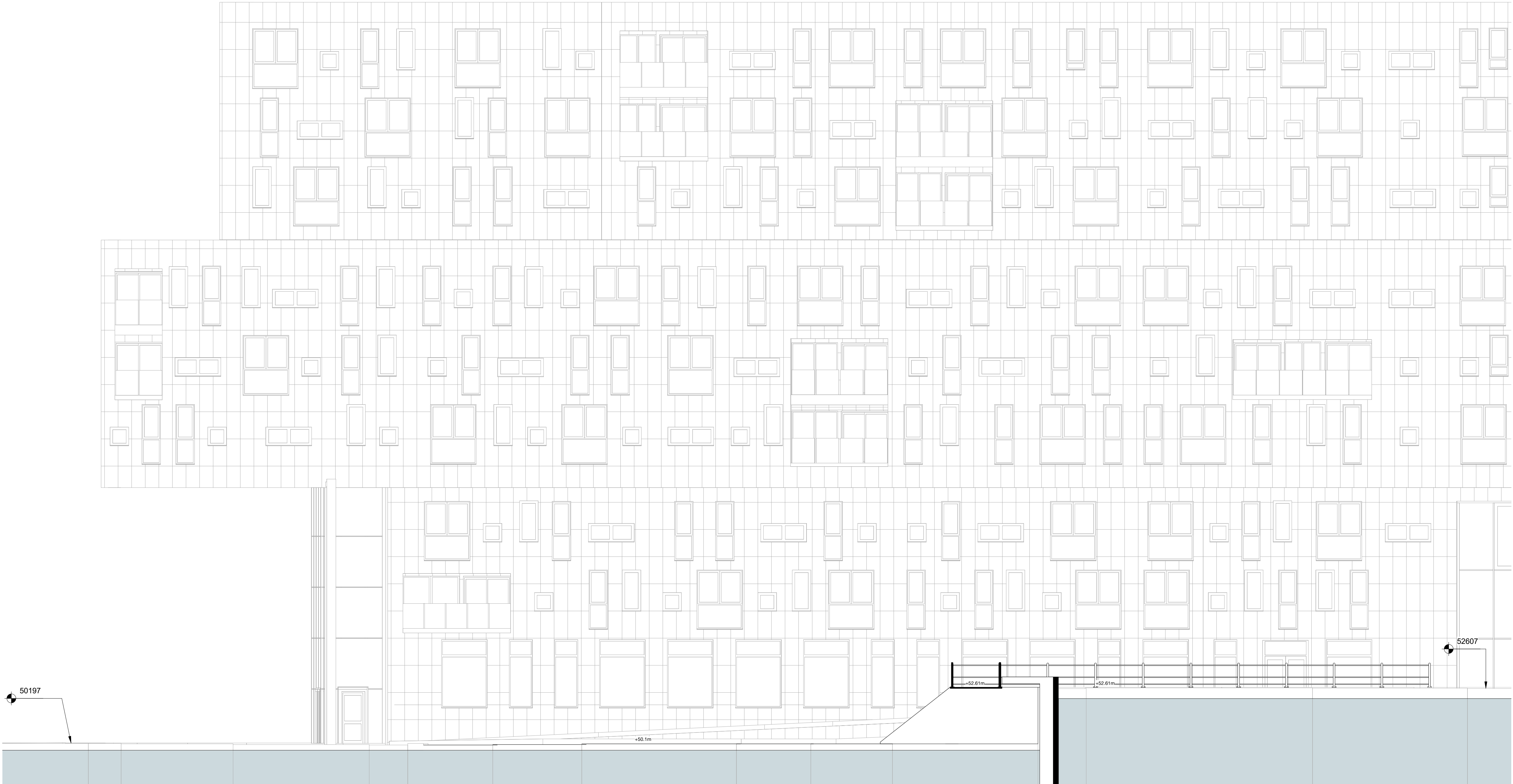
Existing Elevation A-A 1 : 100
