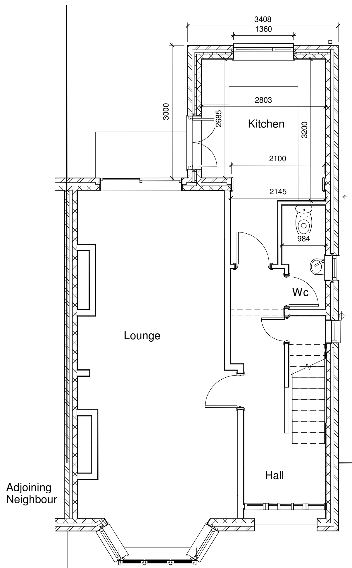
01 Proposed Ground Floor Plan 1 : 50
