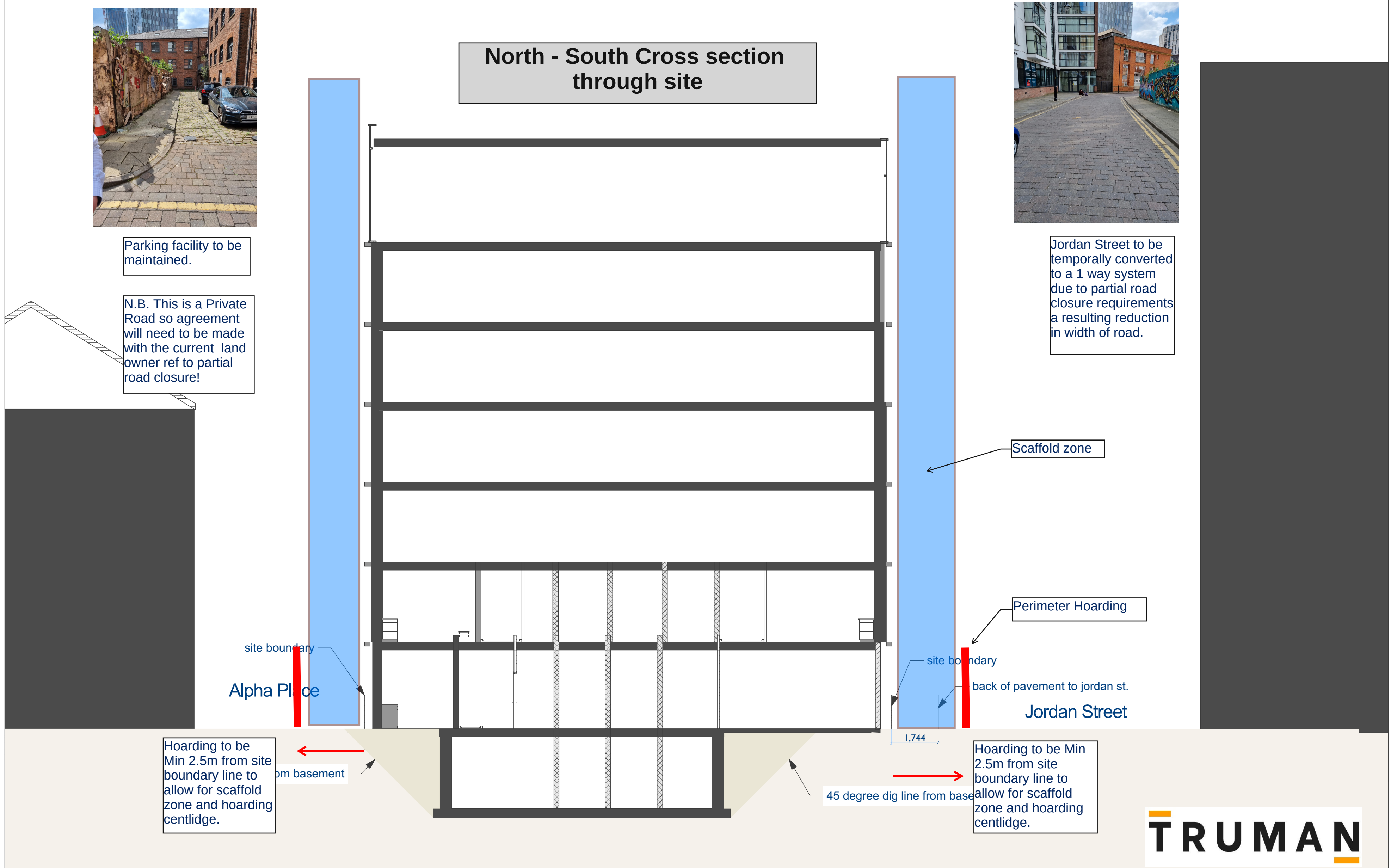
Cross Section Through Site
