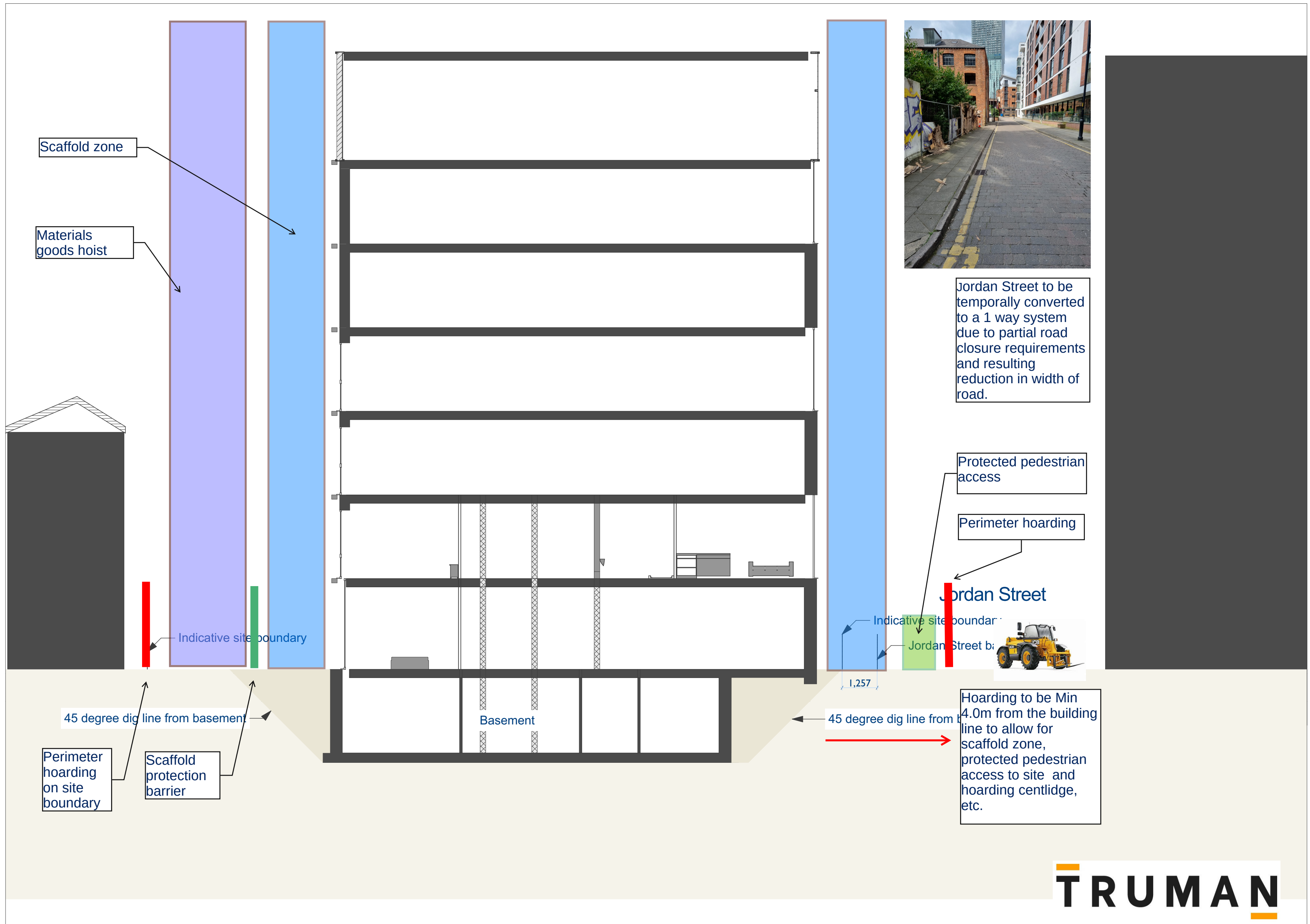
Cross Section Through Site
