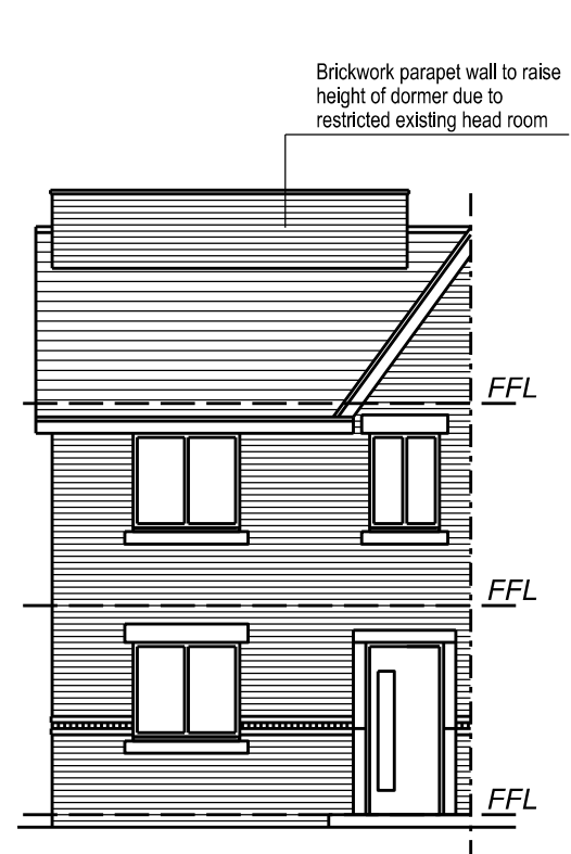
South Elevation
