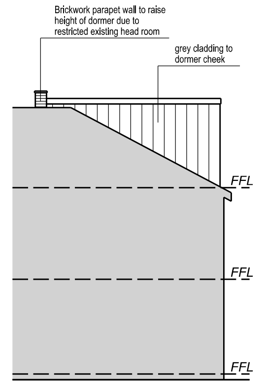
East Elevation
