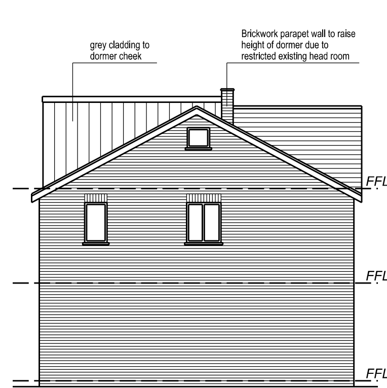
West Elevation
