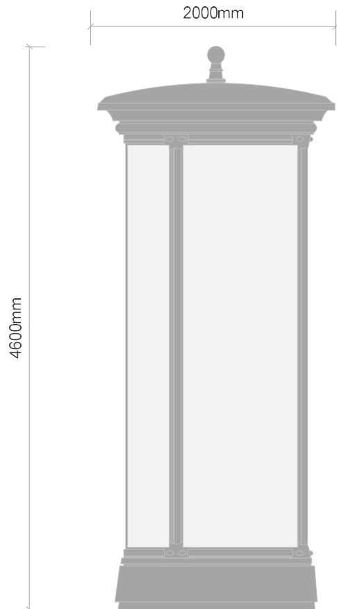
Existing Column Structure
