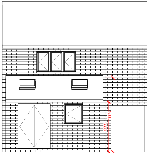
3 Rear Proposed 1 : 100
