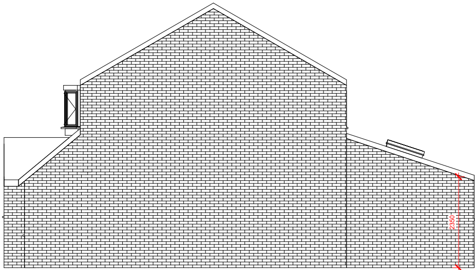
4 Right Proposed 1 : 100
