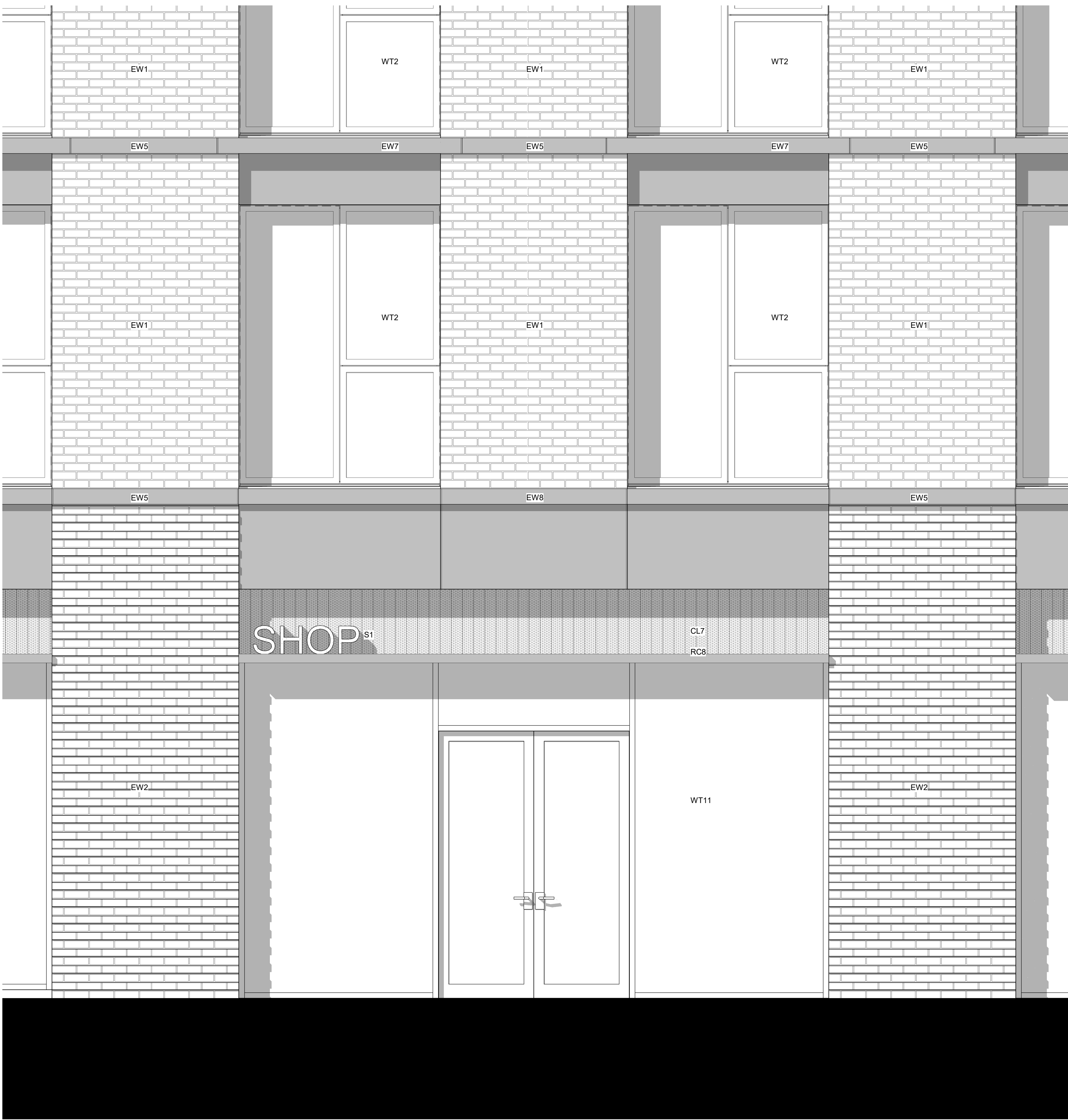
Commercial Bay & Typical Residential Window_Planning 1 : 20
