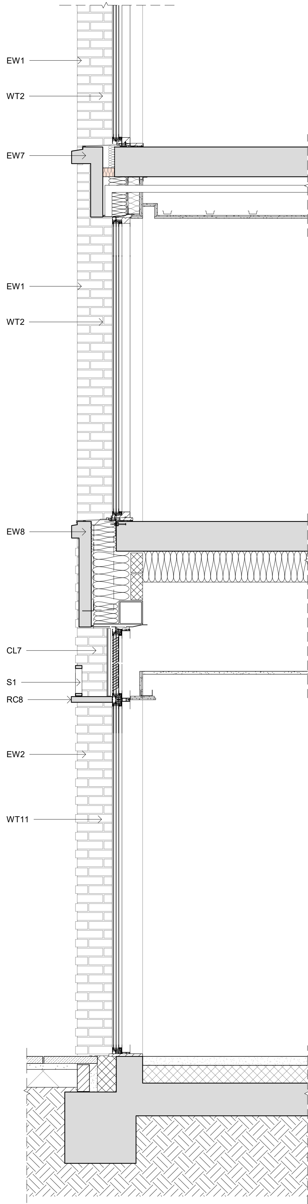
1-20 Detail Sections - Commercial Bay_Planning 1 : 20
