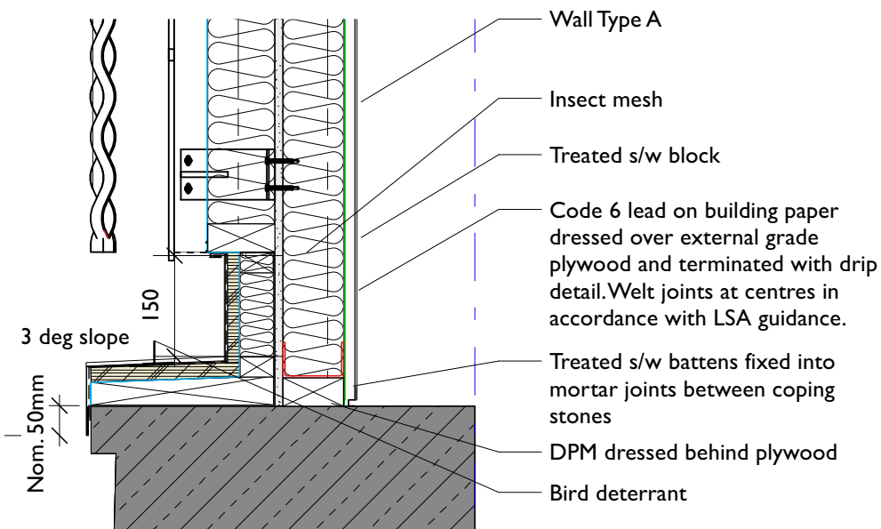
2 Junction New Wall to Stone Parapet Scale: 1:10
