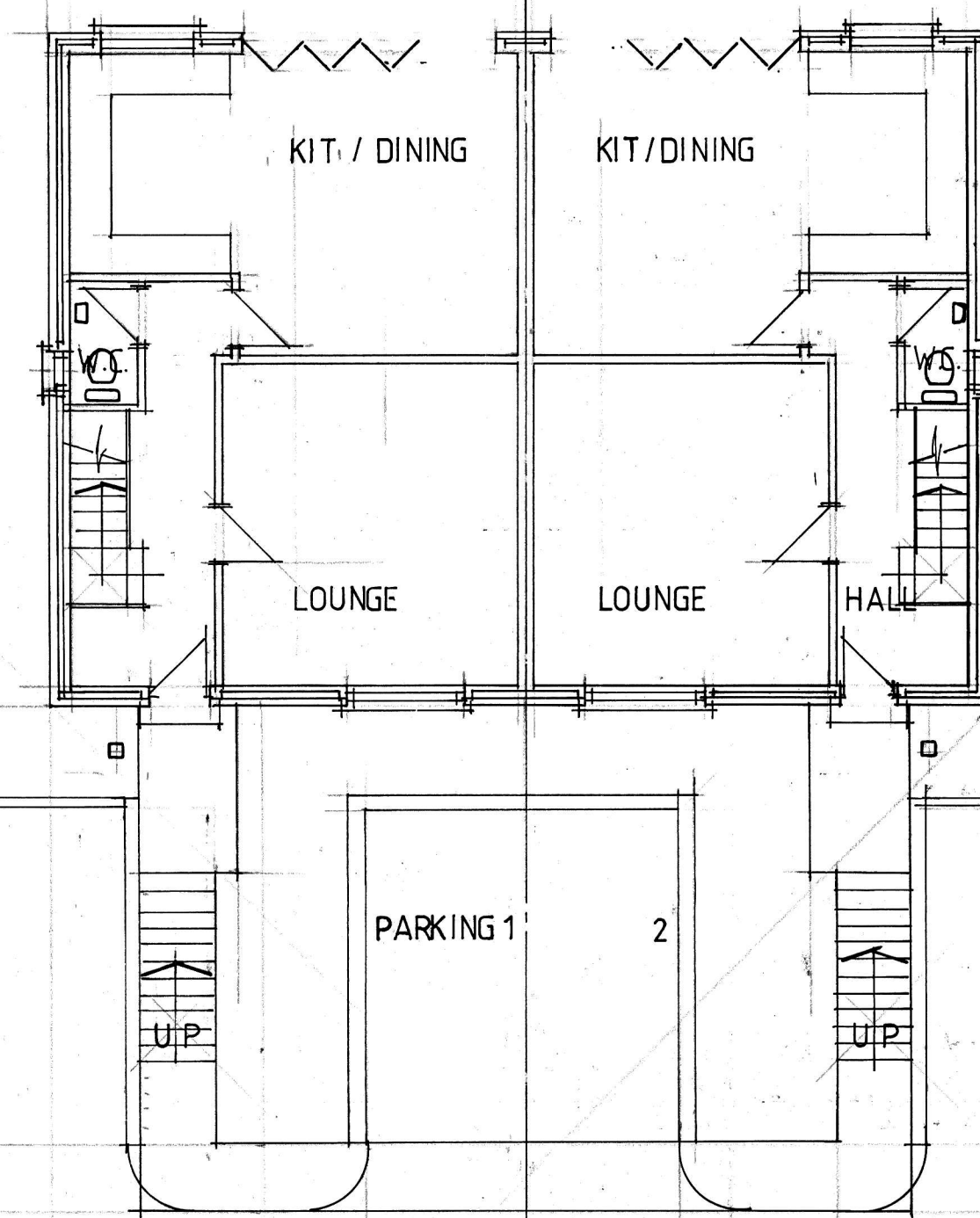
Ground Floor
