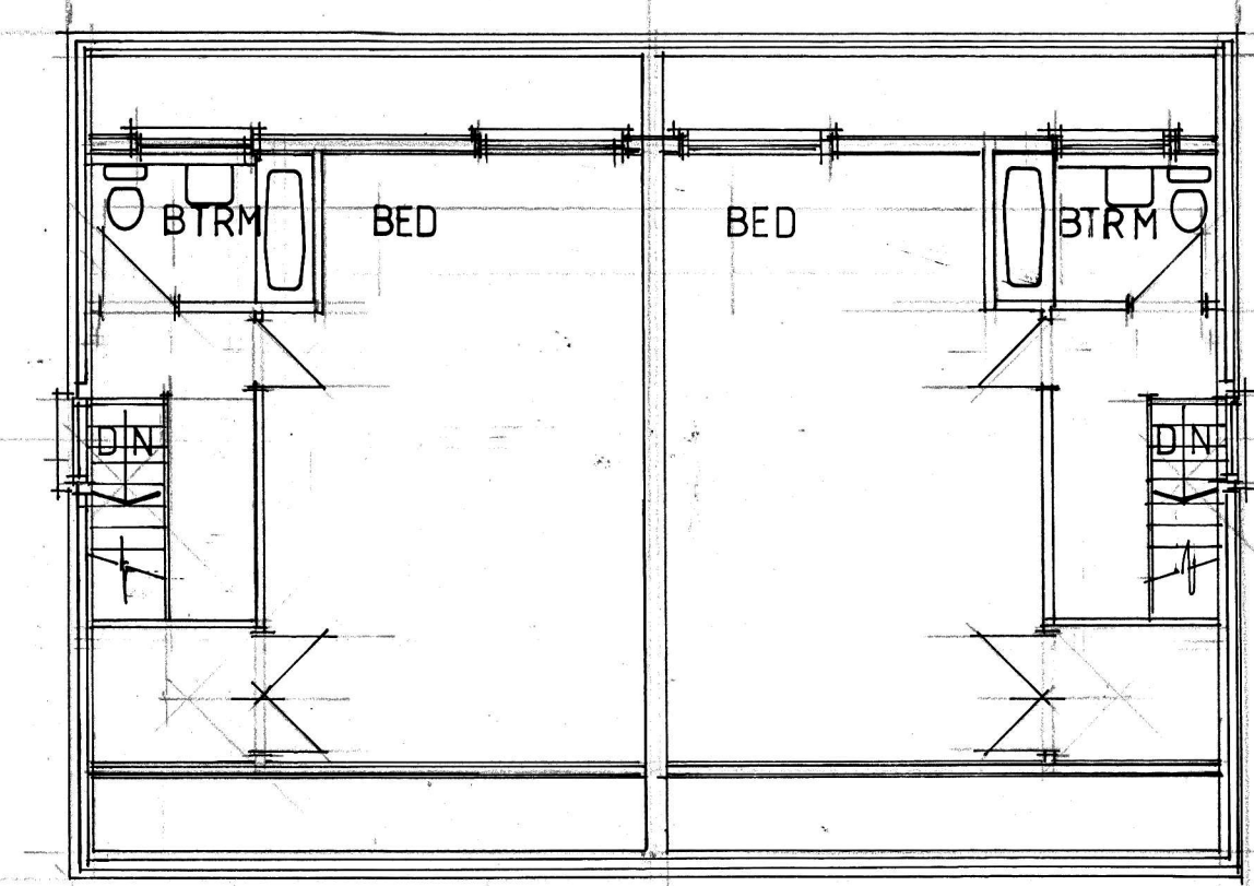
Second Floor
