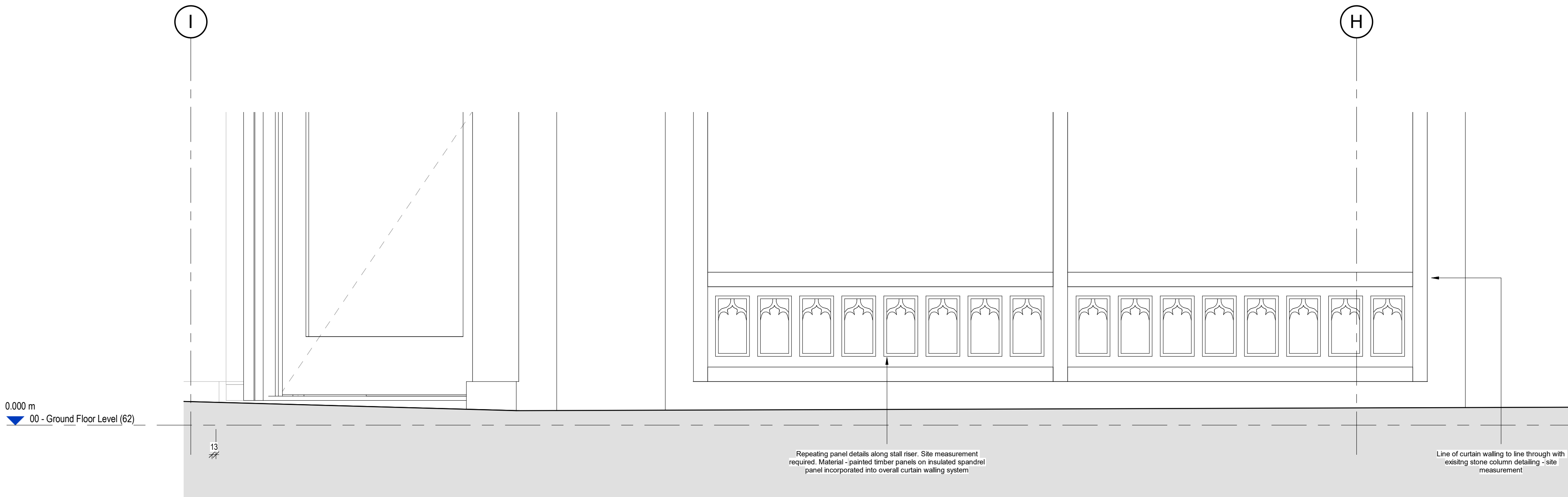
2 Proposed Elevation 2 Lobby Stall Riser Detail Scale @ 1 : 10
