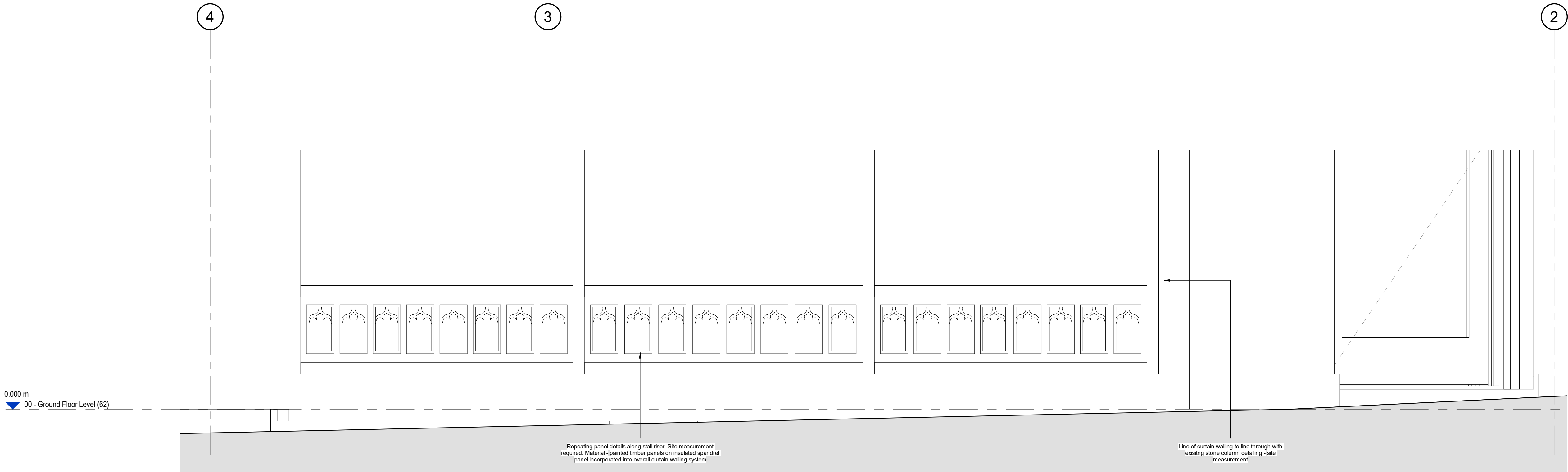
1 Proposed Elevation 1 Lobby Stall Riser Detail Scale @ 1 : 10
