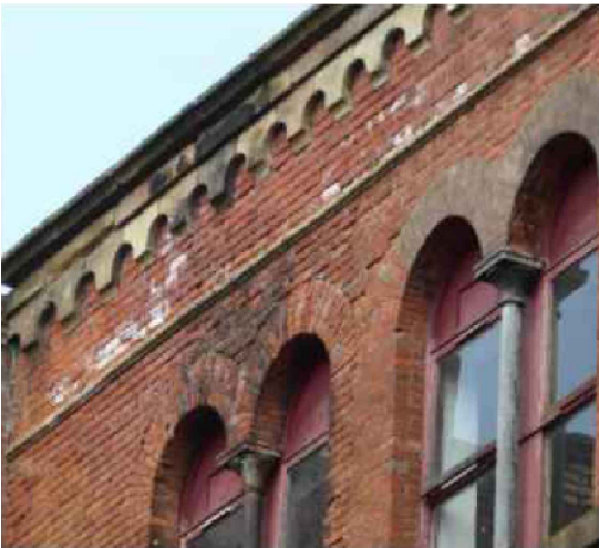
2. Water staining on cornice. Investigate cause and clean. Repoint brickwork with mortar to match existing if necessary.
